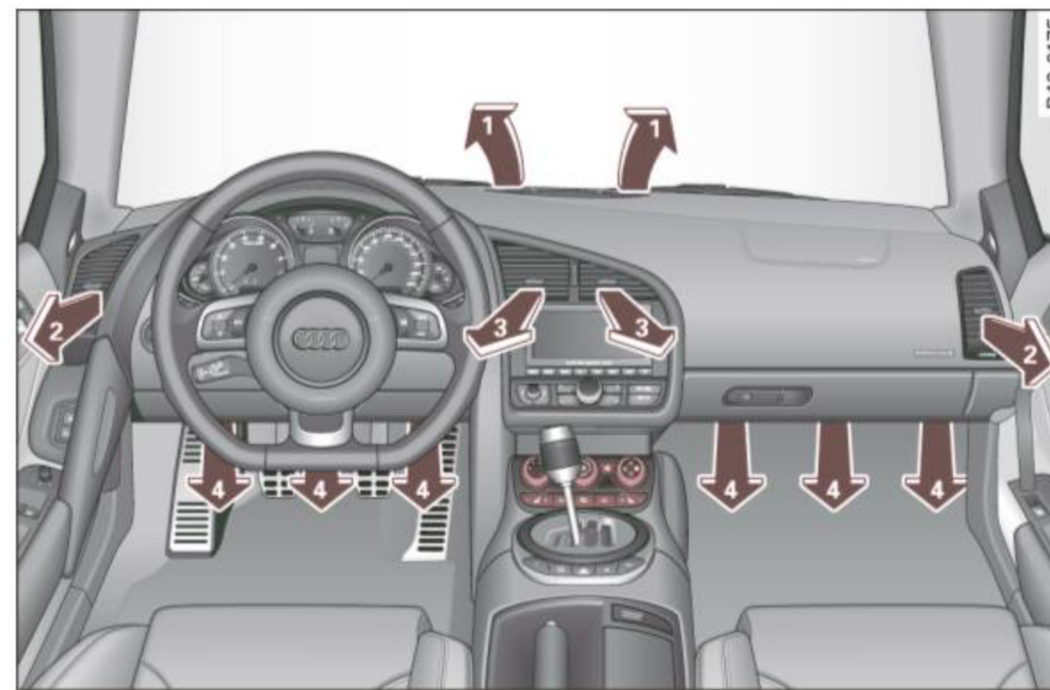
Fig. 61 Instrument panel: Location of air vents
