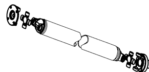
21600 前桥传动轴 Front Axle Drive Shaft
