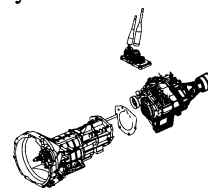
20800 变速器带分动器总成 Transmission With Transfer Case Assembly
