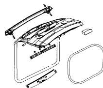
70600 后背门总成 Tailgate Assembly
