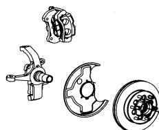
40700 前轮毂及转向节 Front Wheel Hub And Steering Knuckle
