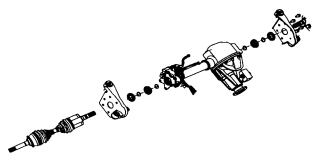
30500 后桥壳及半轴 Rear Axle Housing And Halfaxle
