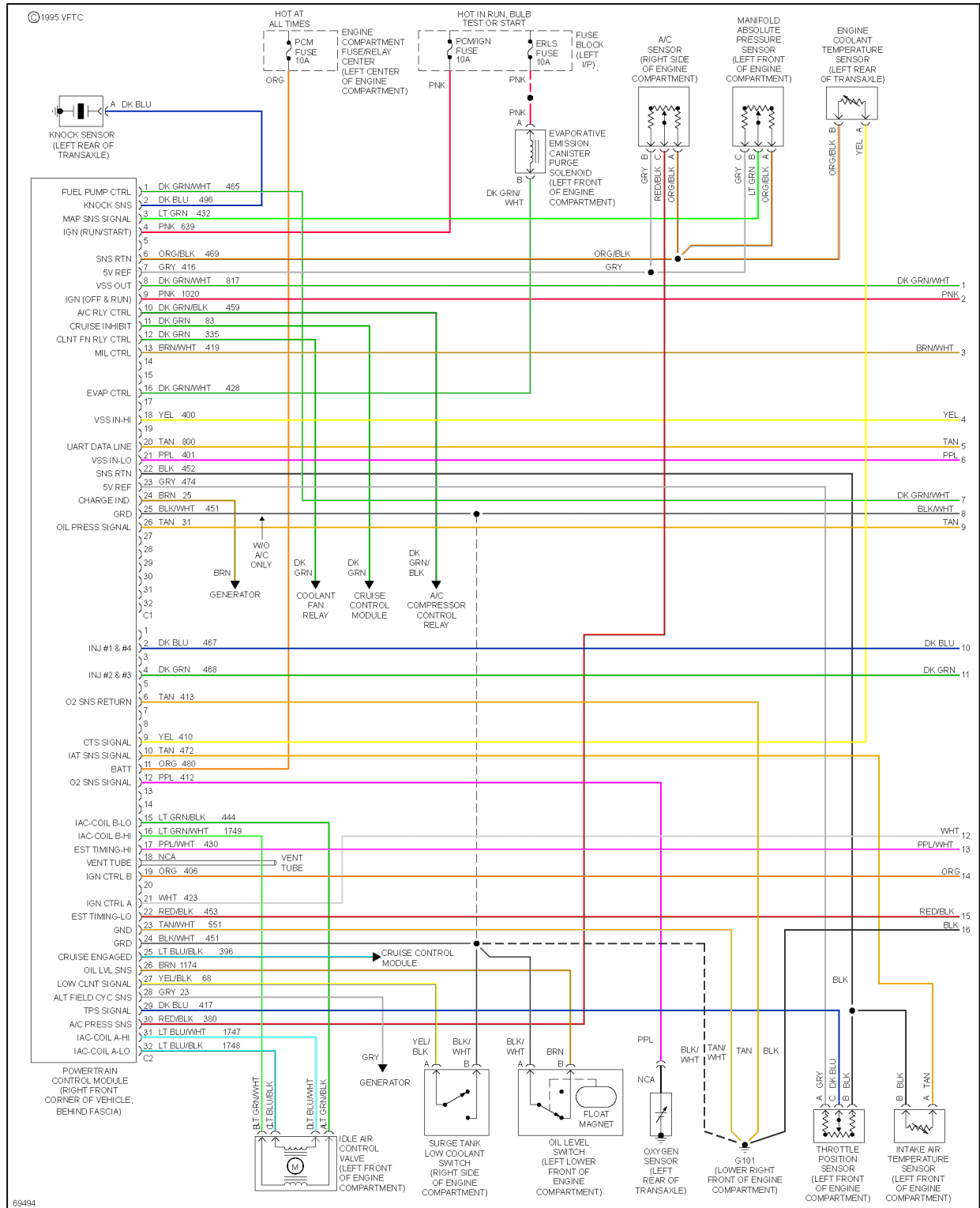
Fig. 15: 2.3L (VIN D), Engine Performance Circuits, M/T (1 of 2)
