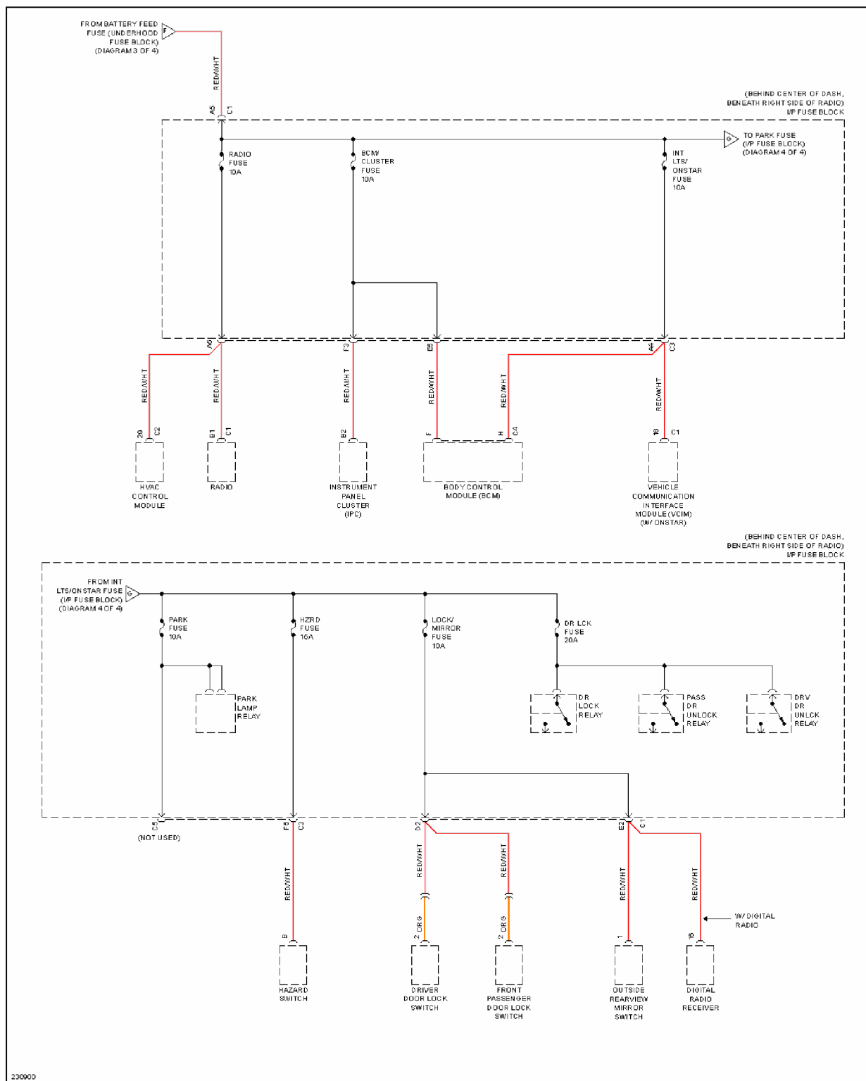
Fig. 30: Power Distribution Circuit (4 of 4)
