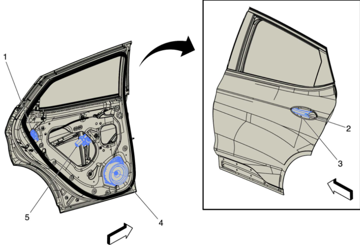
Fig. 5: Left Rear Door Components Courtesy of GENERAL MOTORS COMPANY
