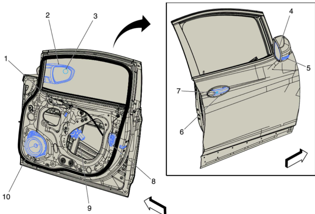
Fig. 3: Passenger Door Components
