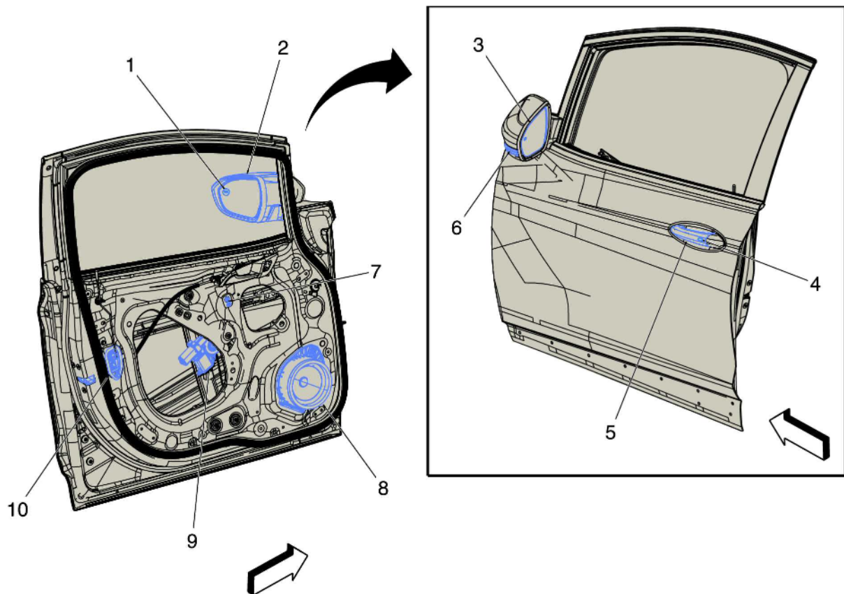
Fig. 1: Driver Door Components
