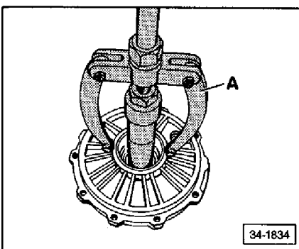
► Fig. 6 Differential bearing, large — outer race, removing
