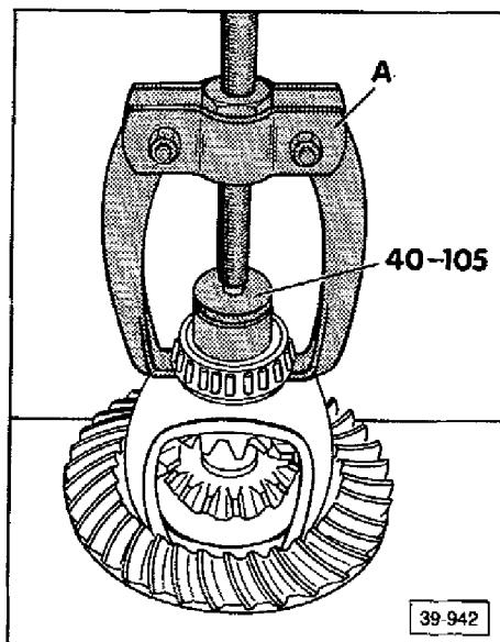
► Fig. 3 Differential bearing, small — inner race, removing
