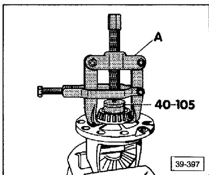
► Fig. 5 Differential bearing, large — inner race, removing
