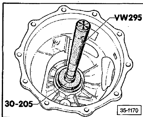
► Fig. 2 Differential bearing, small — outer race, installing
