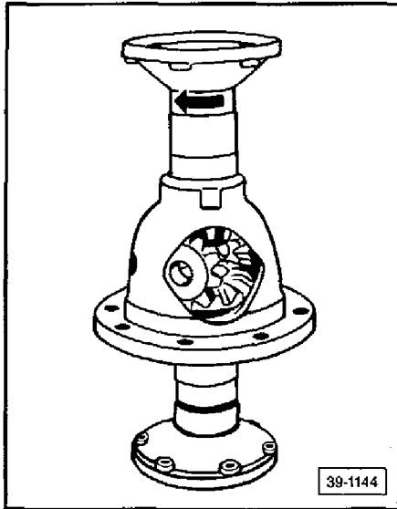
► Fig. 7 Differential gears, installing
