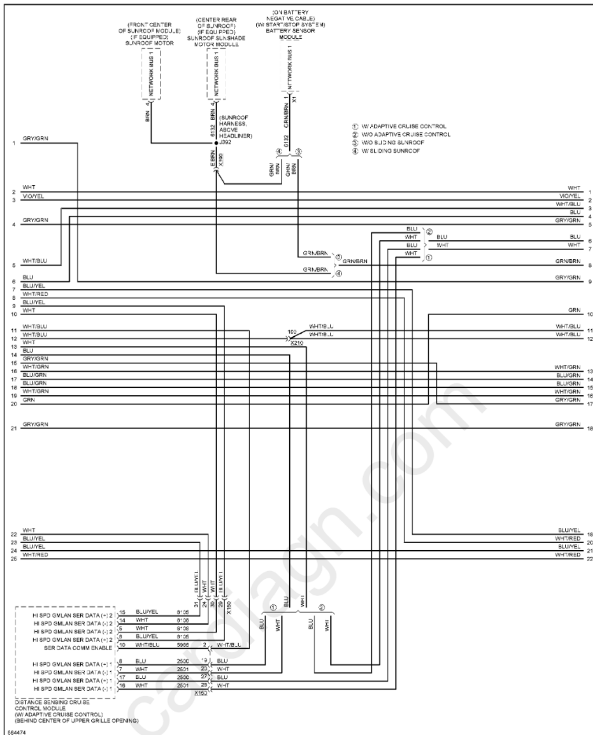
Fig. 23: Computer Data Lines Circuit (3 of 7)
