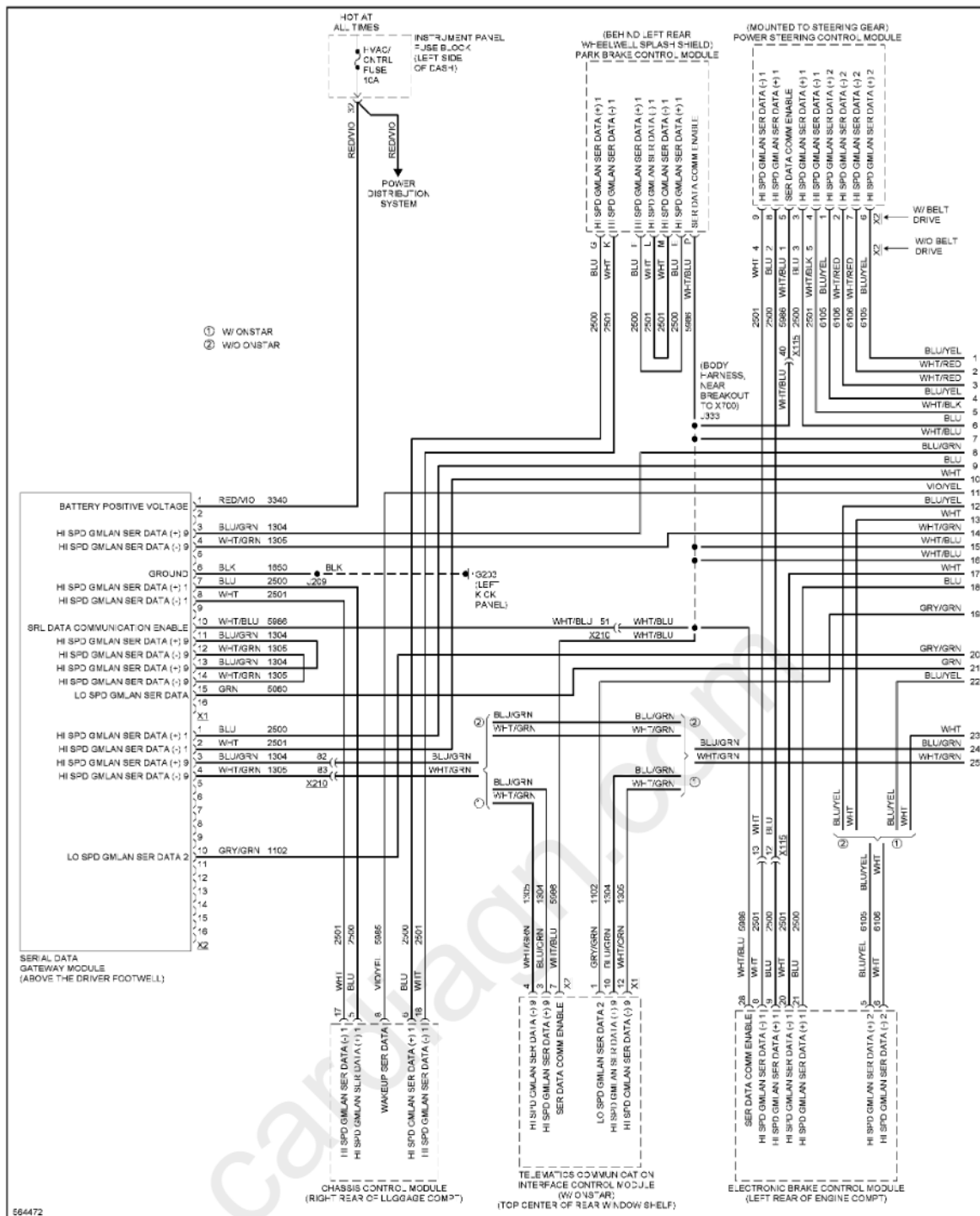
Fig. 21: Computer Data Lines Circuit (1 of 7)
