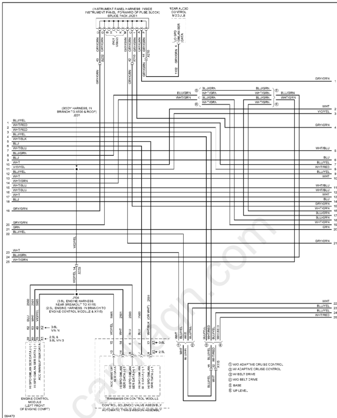
Fig. 22: Computer Data Lines Circuit (2 of 7)
