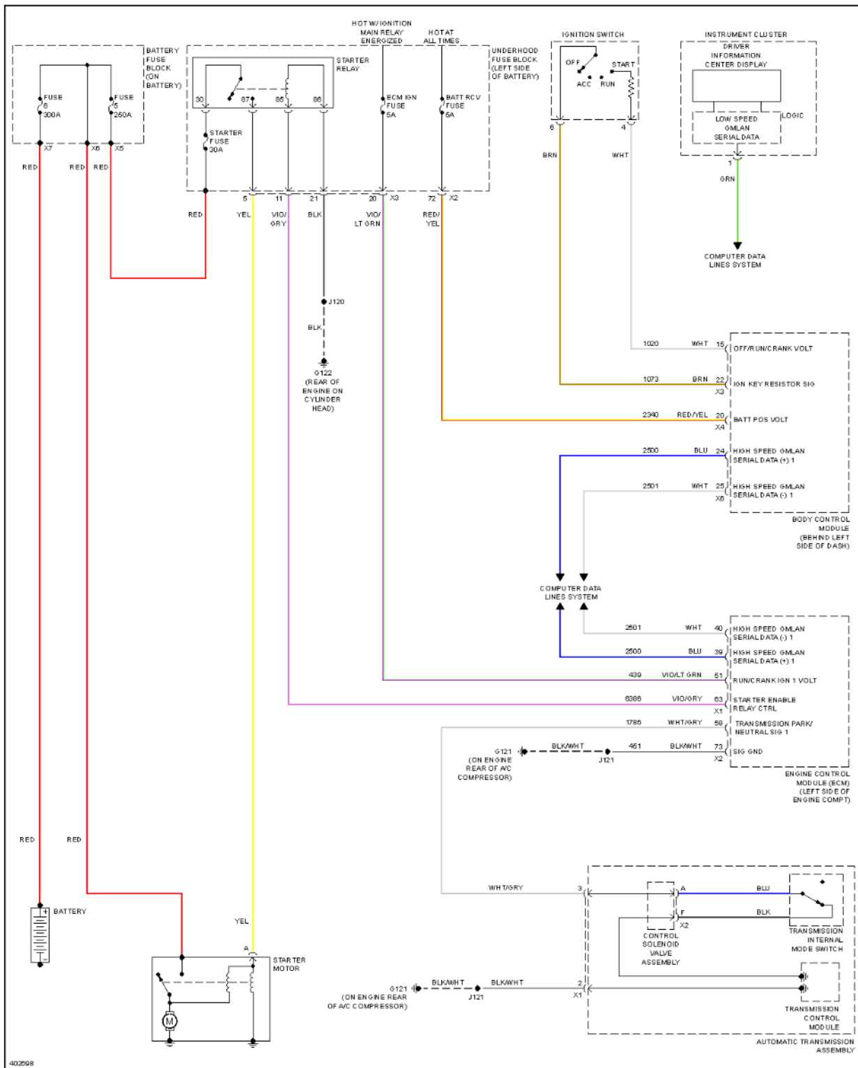
Fig. 126: Starting Circuit, Hybrid
