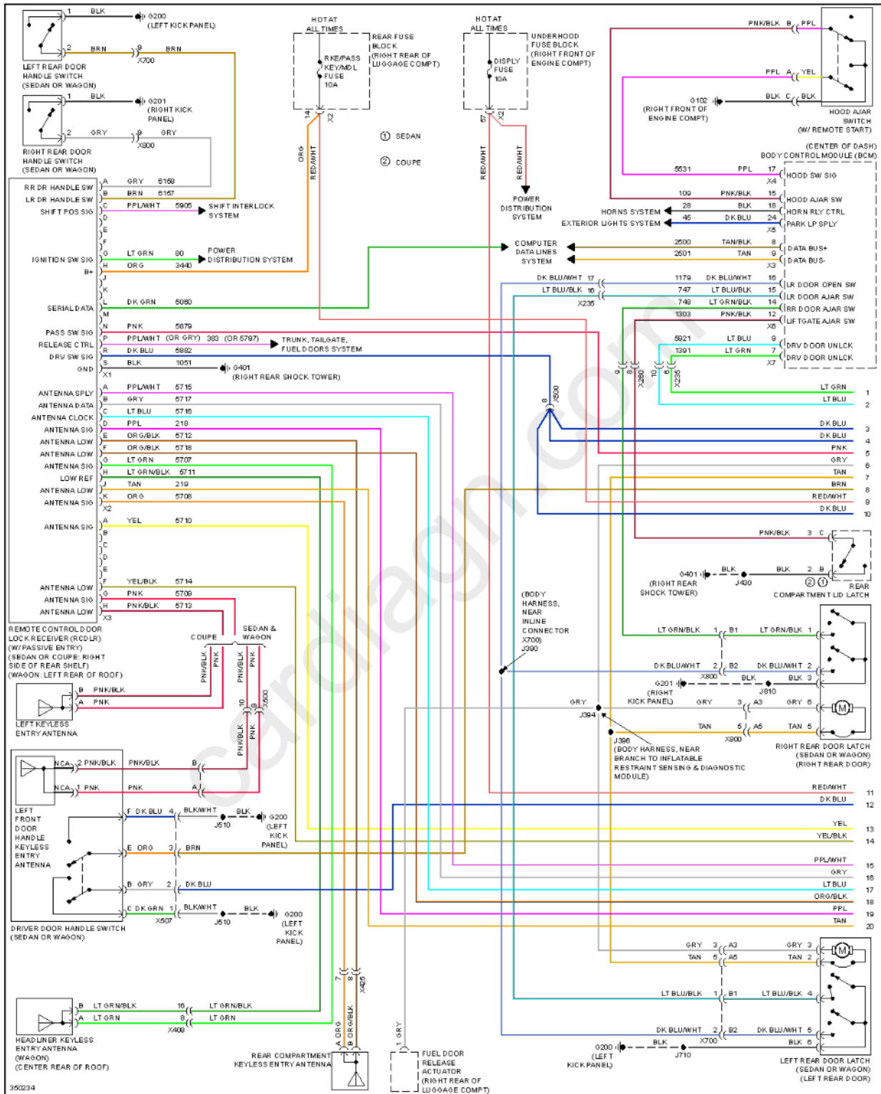
Fig. 6: Forced Entry Circuit (1 of 3)
