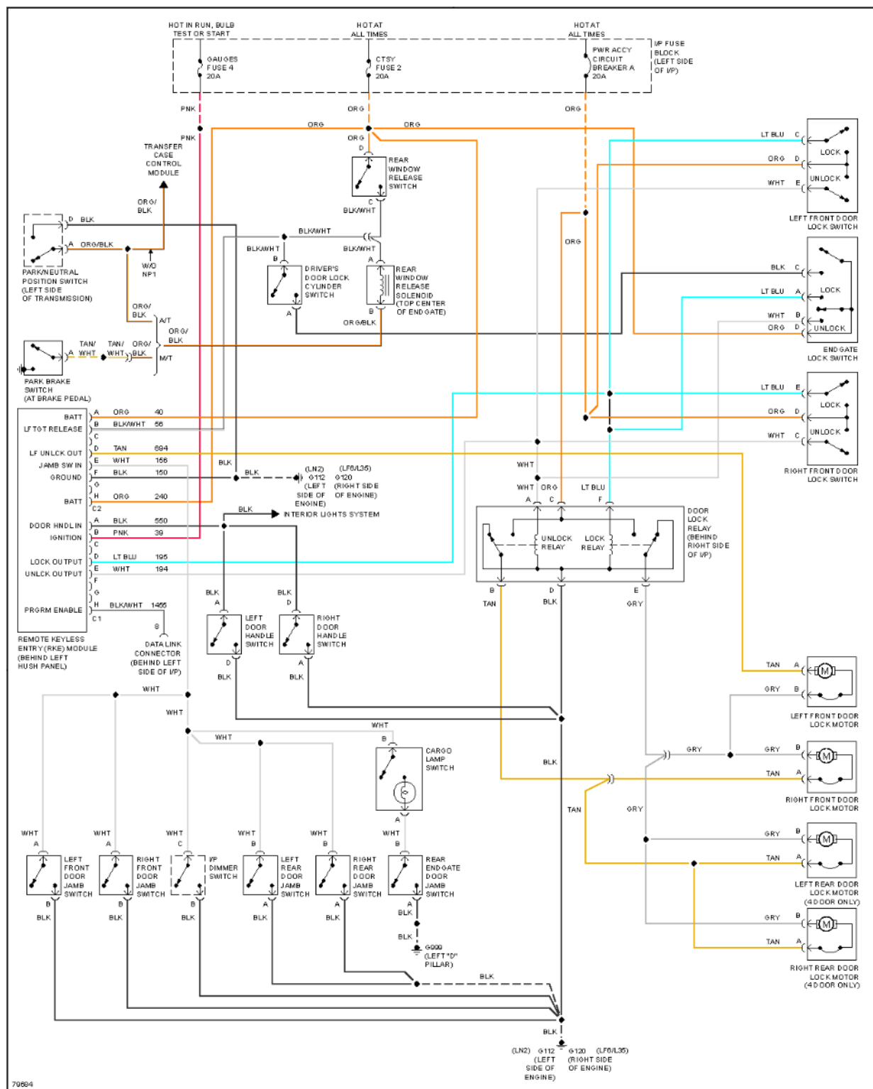
Fig. 24: Keyless Entry Circuit
