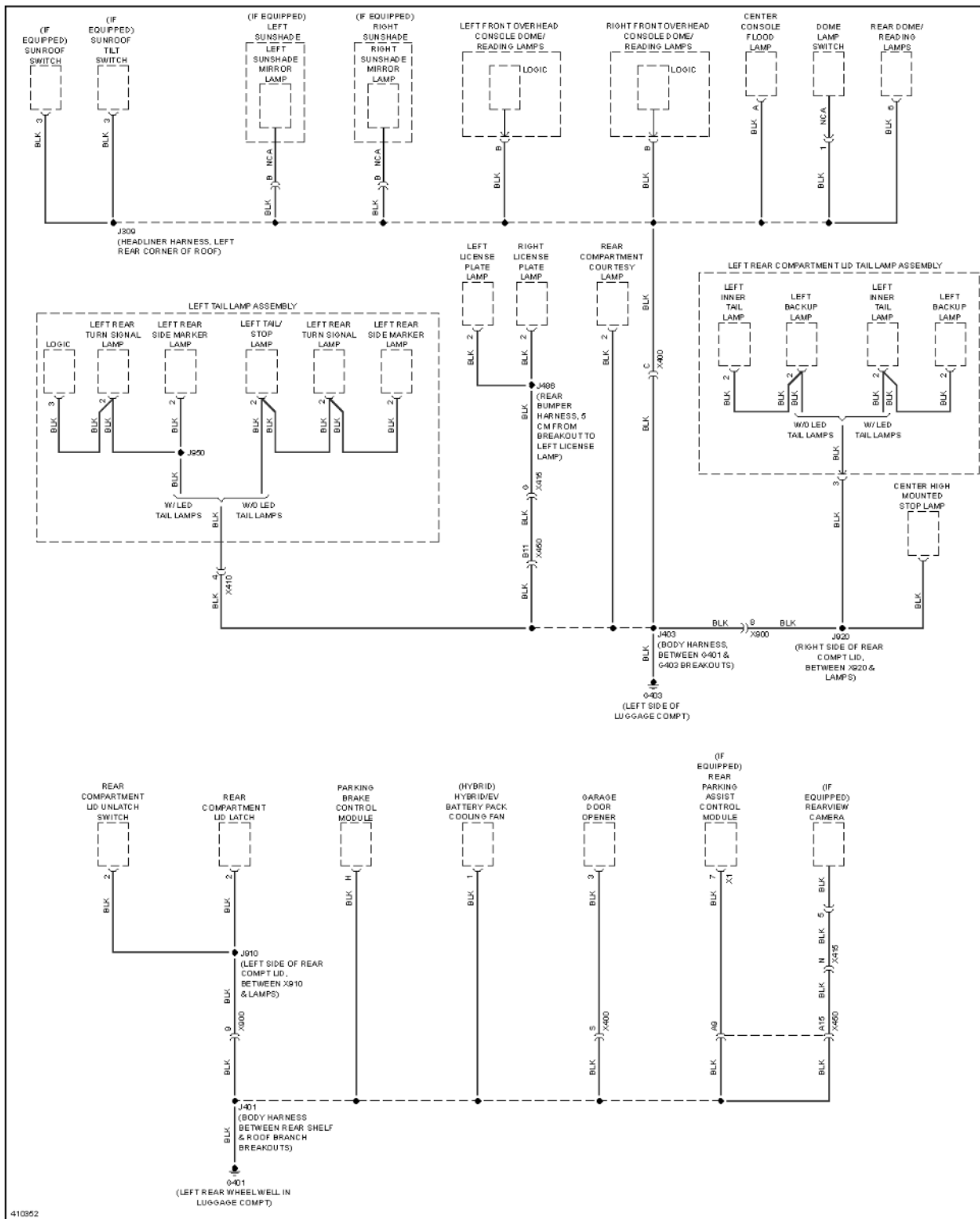
Fig. 60: Ground Distribution Circuit (6 of 6)
