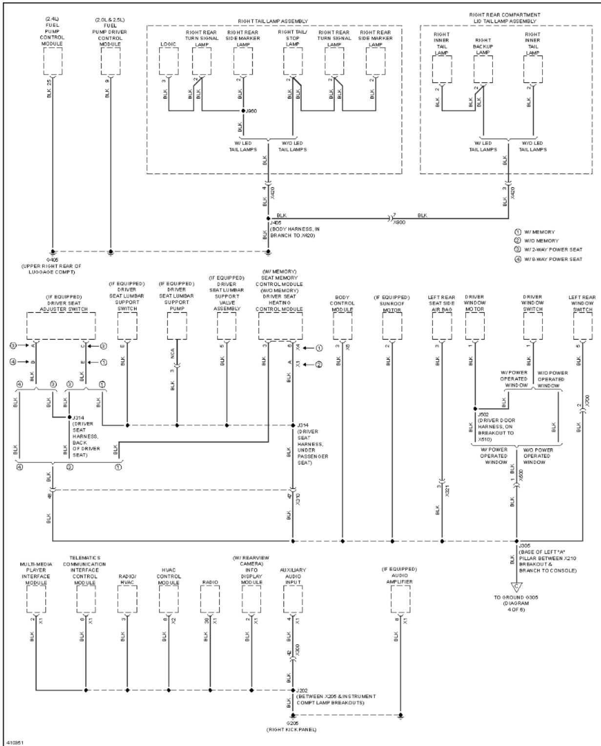
Fig. 59: Ground Distribution Circuit (5 of 6)
