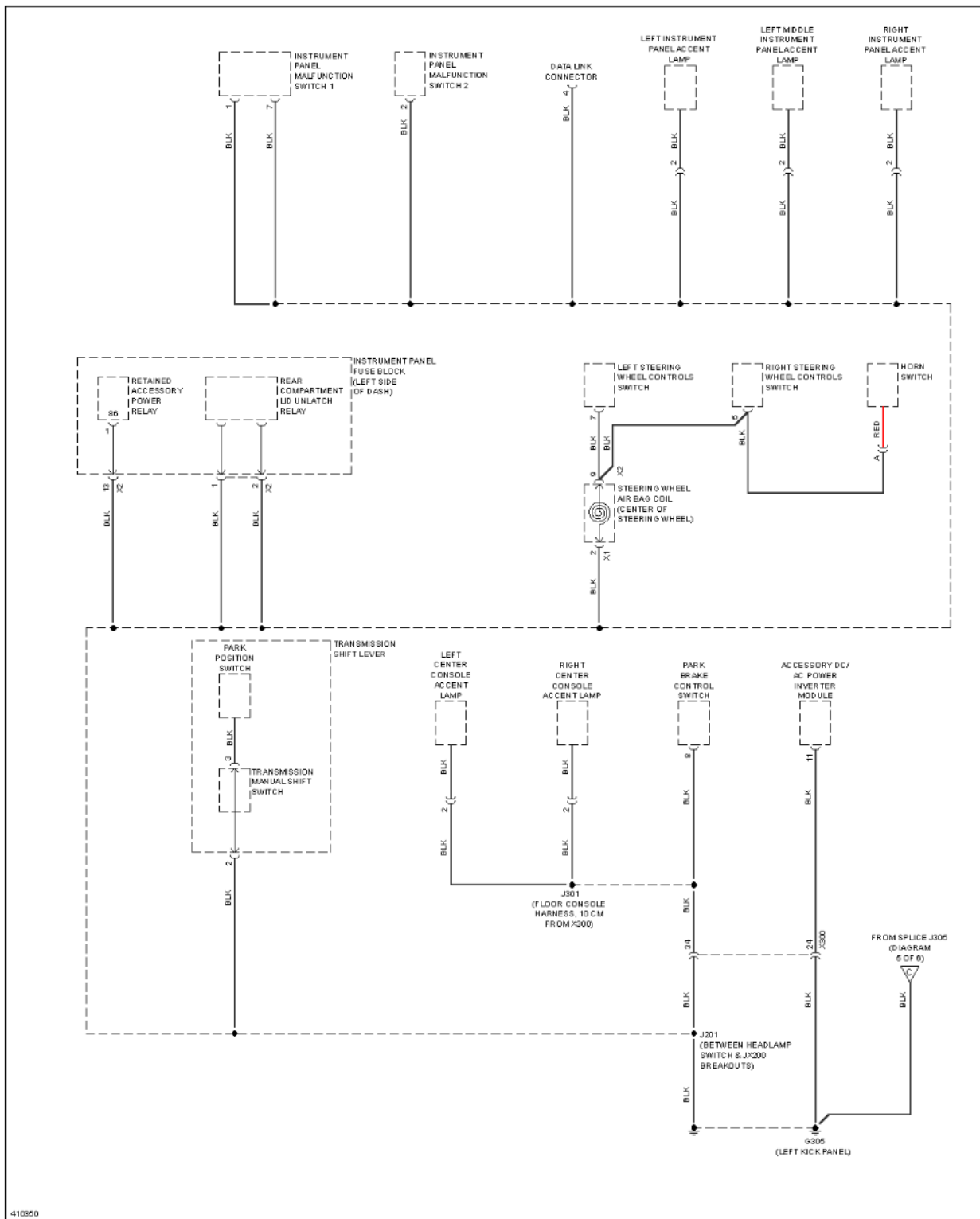
Fig. 58: Ground Distribution Circuit (4 of 6)
