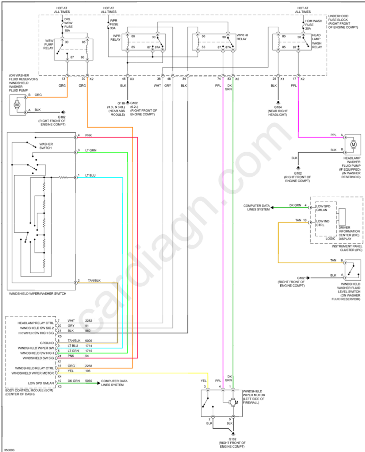
Fig. 121: Wiper/Washer Circuit, Coupe
