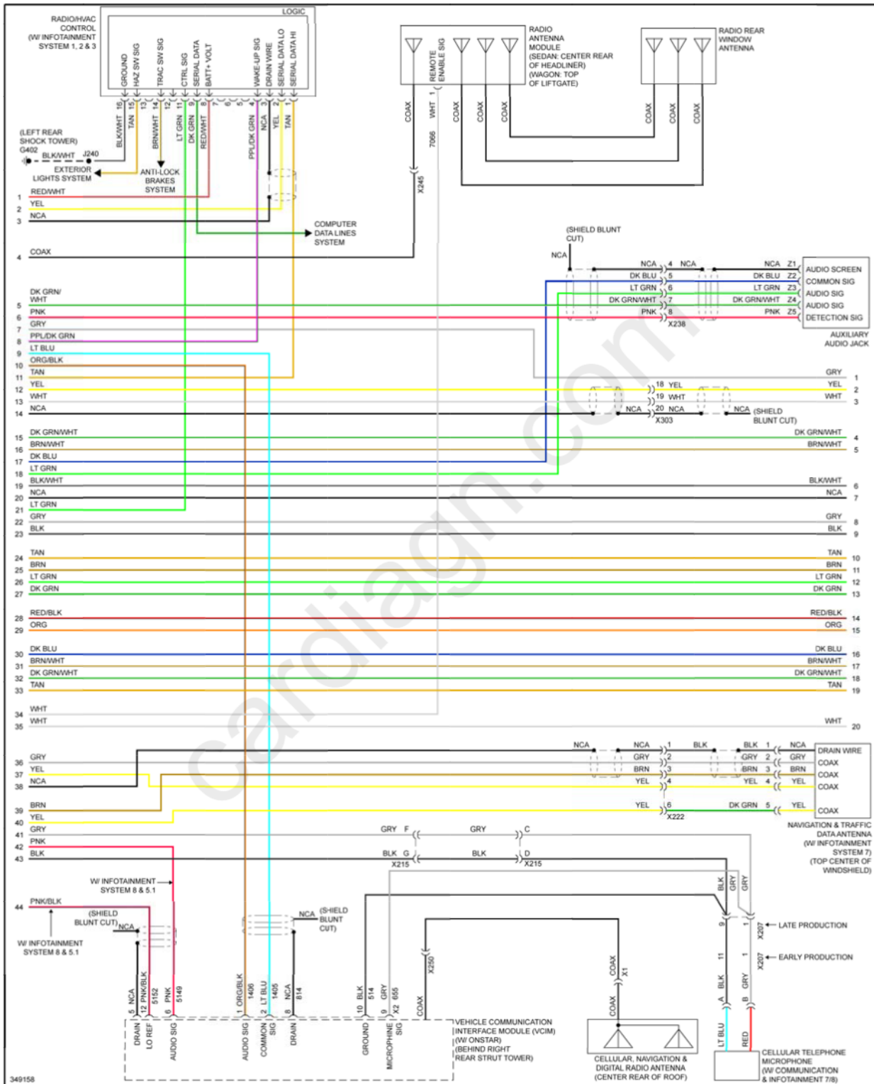
Fig. 104: Radio Circuit, W/O Surround Amplifier (2 of 4)
