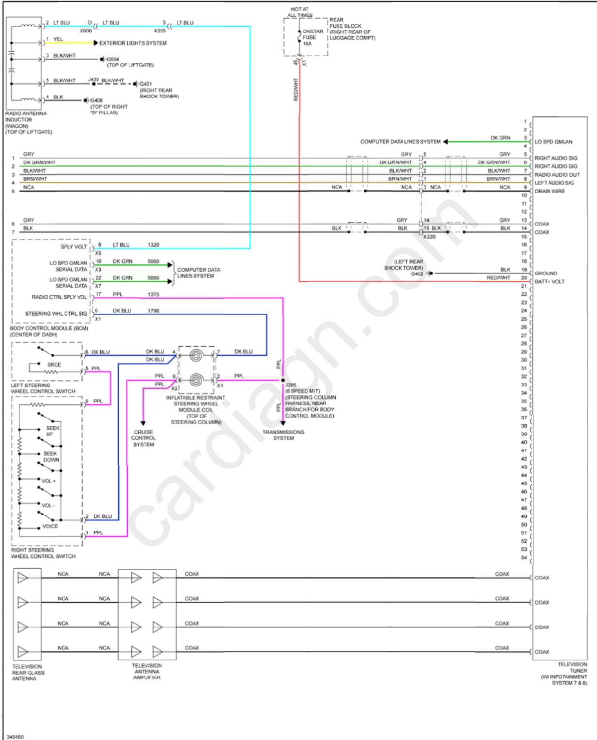
Fig. 106: Radio Circuit, W/O Surround Amplifier (4 of 4)
