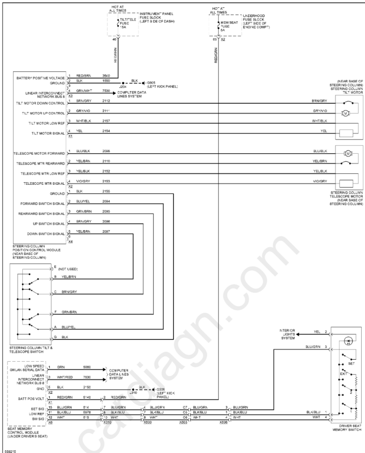
Fig. 74: Memory Power Tilt & Power Telescopic Circuit
