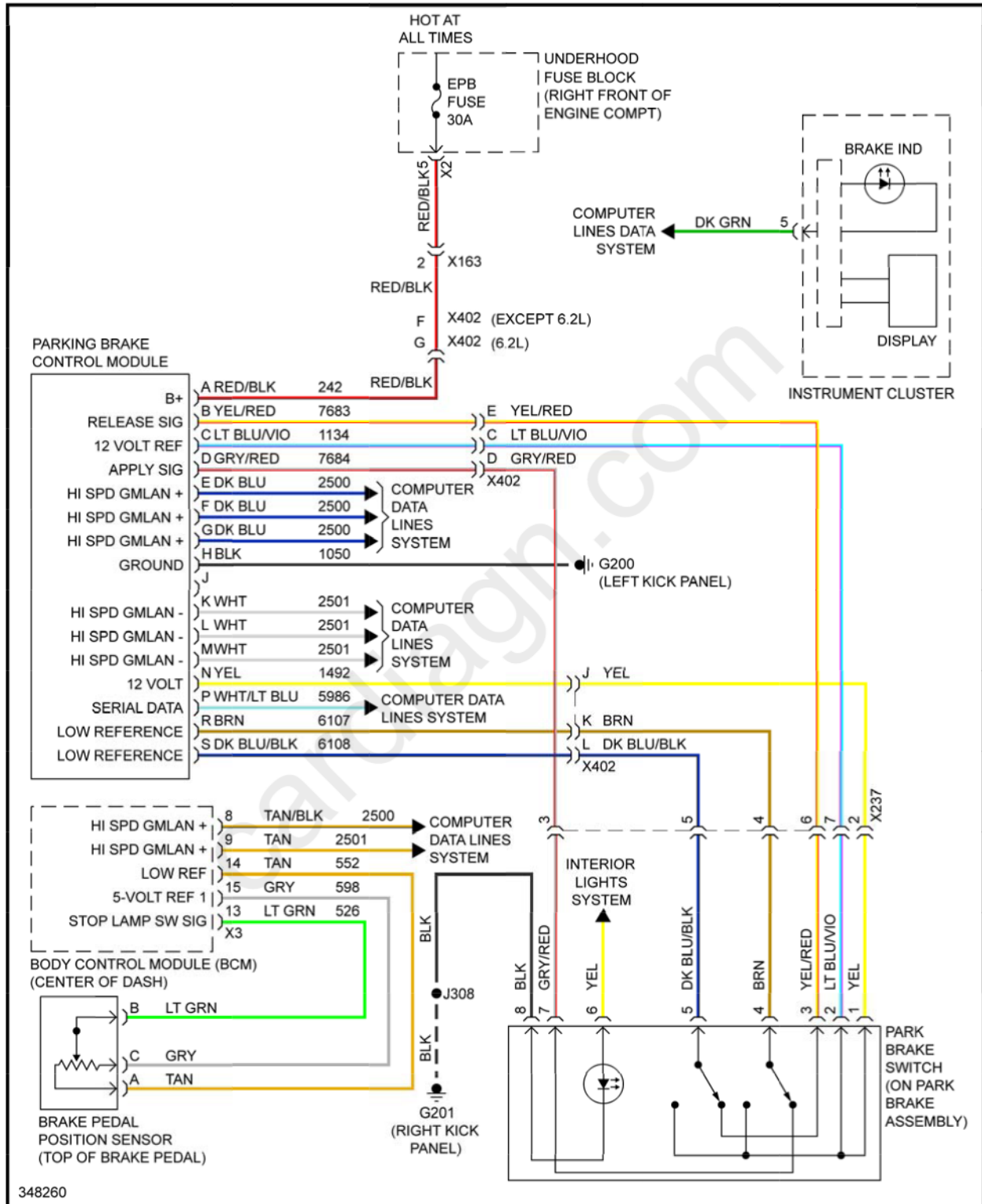
Fig. 109: Park Brake System Circuit
