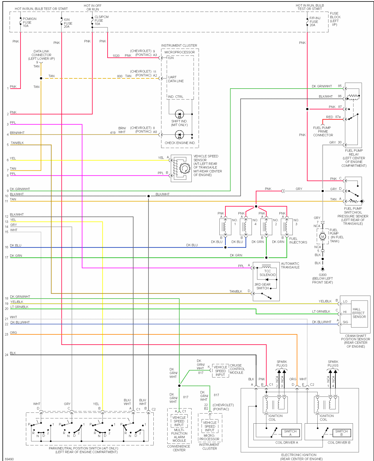
Fig. 11: 2.2L (VIN 4), Engine Performance Circuits (2 of 2)
