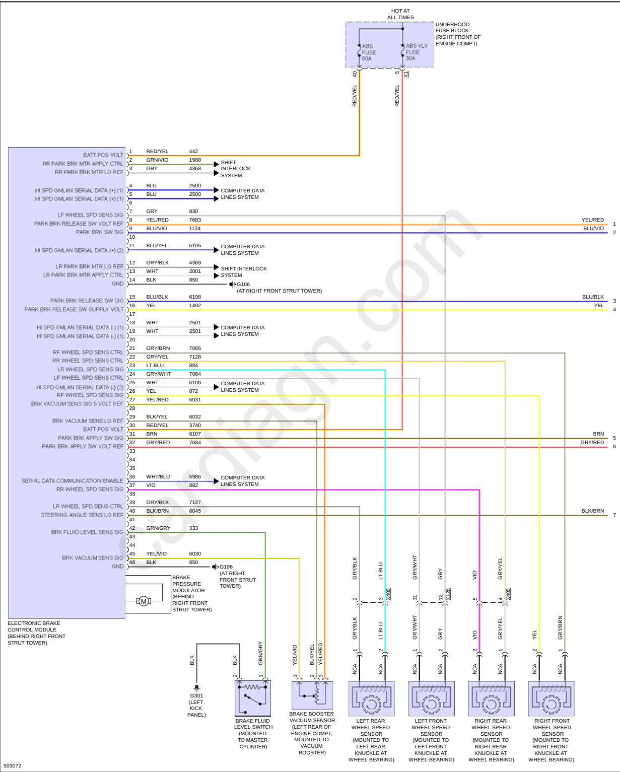
Fig 1: 2.0L VIN X, Anti-lock Brakes Circuit (1 of 2)
