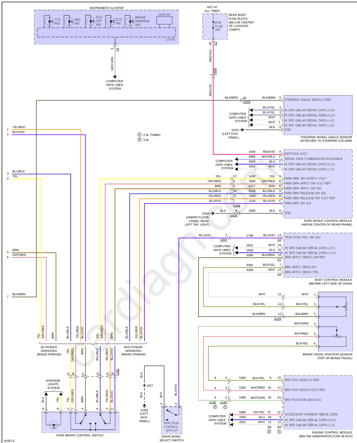
Fig 2: 2.0L VIN X, Anti-lock Brakes Circuit (2 of 2)
