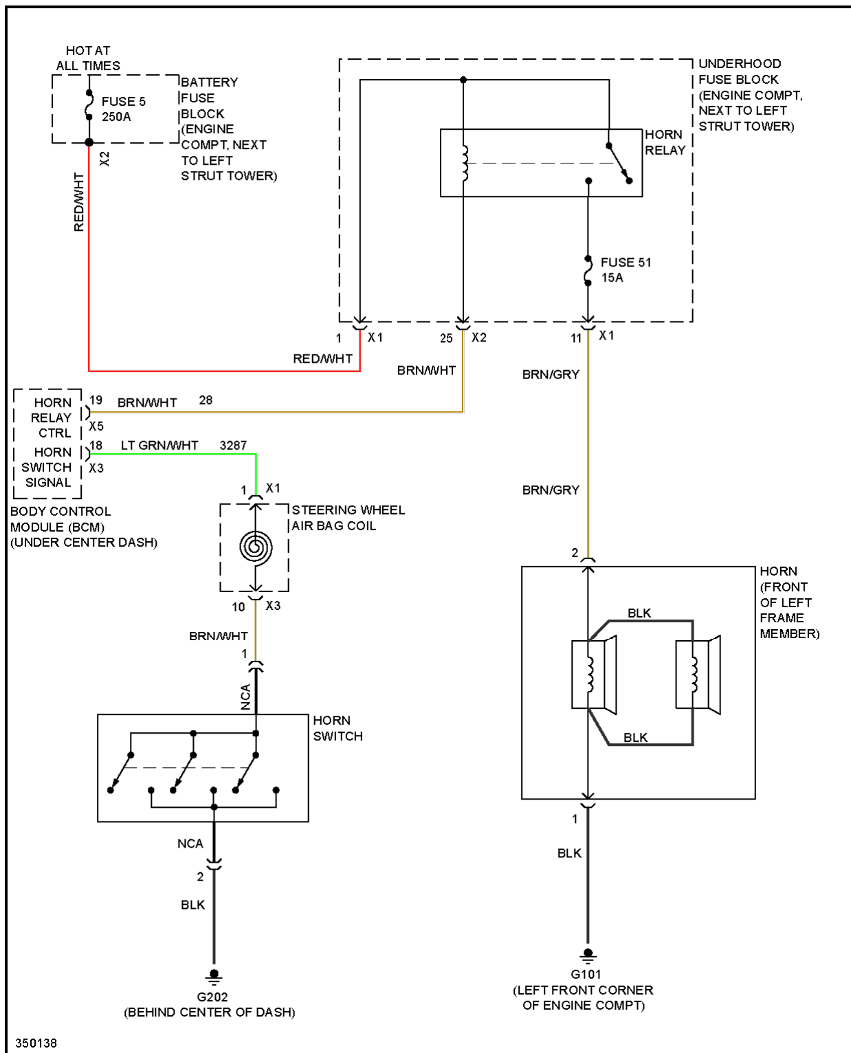
Fig. 35: Horn Circuit
