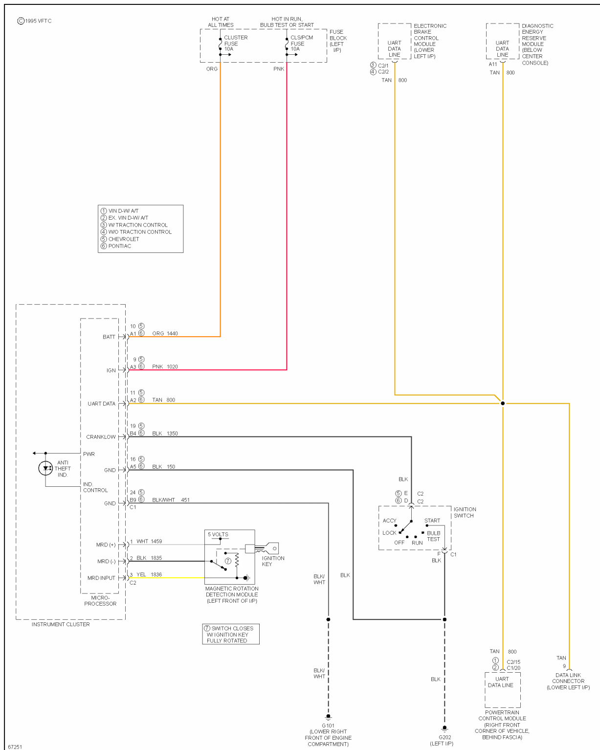
Fig. 5: Passlock Circuit
