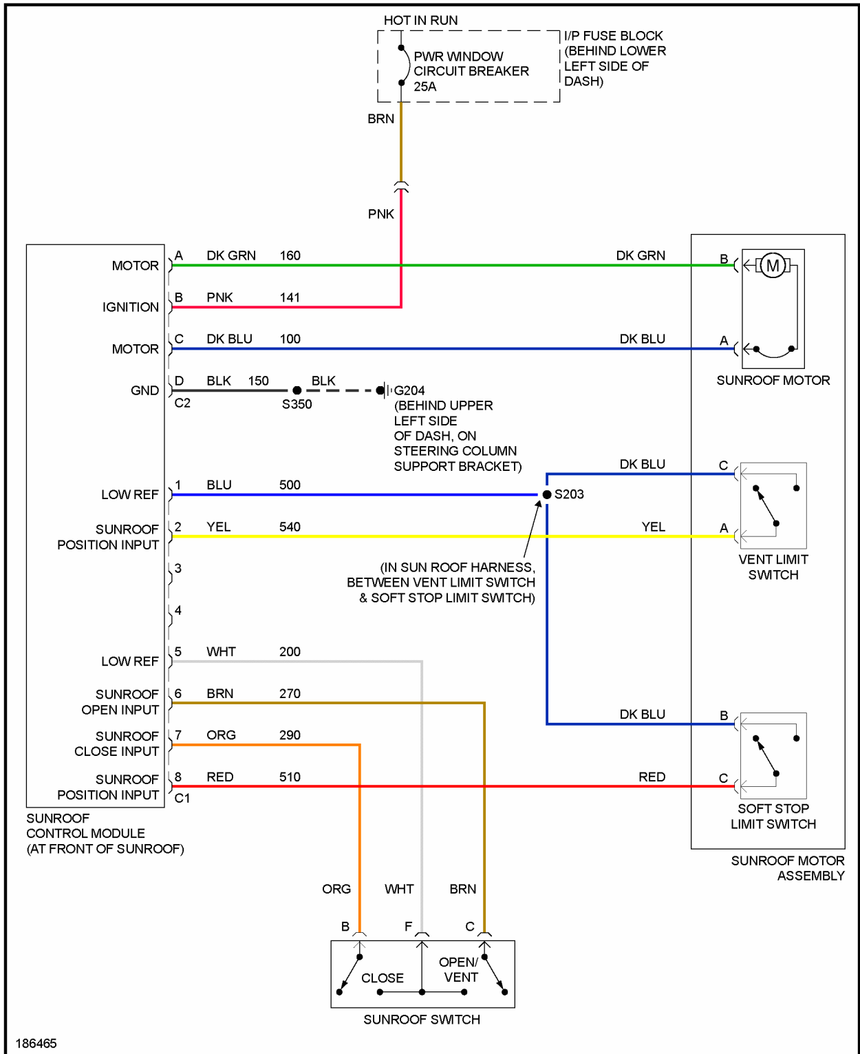
Fig. 27: Power Top/Sunroof Circuit
