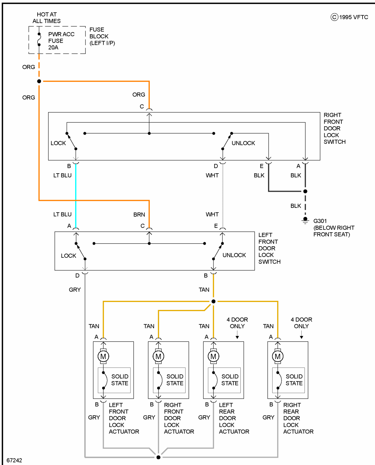
Fig. 32: Power Door Lock Circuit
