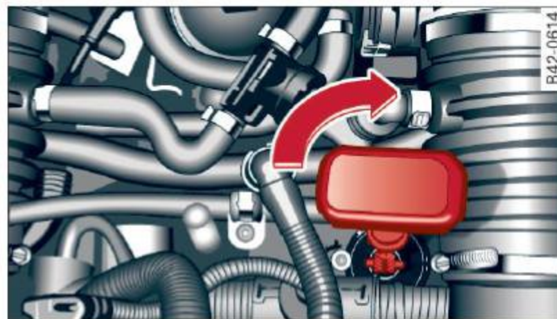
Fig. 87 Engine compartment: parking lock emergency release
