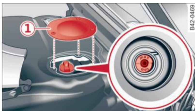
Fig. 145 Convertible top storage bay: coolant expansion tank
