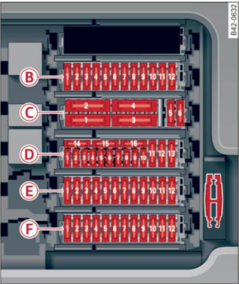
Fig. 167 Passenger footwell: Fuse panel
