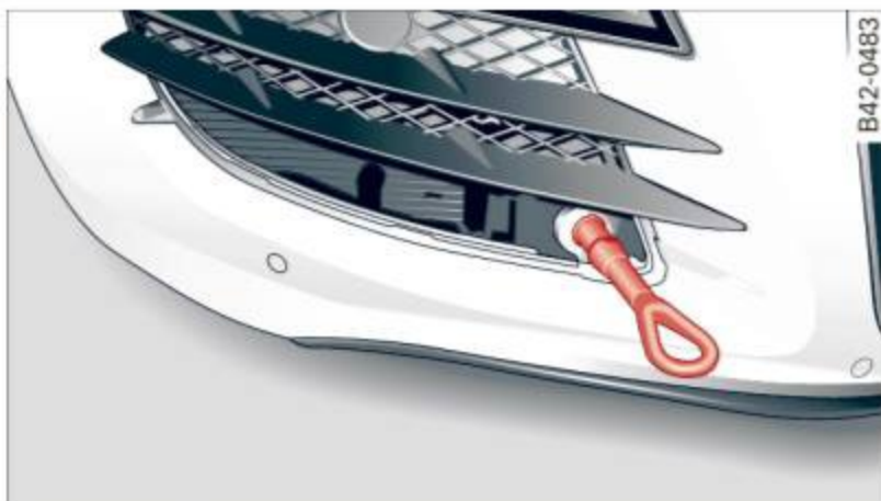
Fig. 165 Right front bumper without grille: Towing loop fully screwed in
