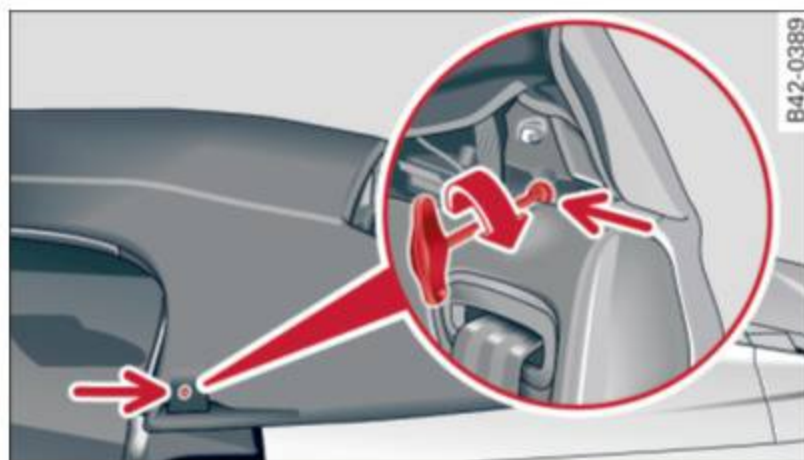
Fig. 50 Interior: tightening the bolt
