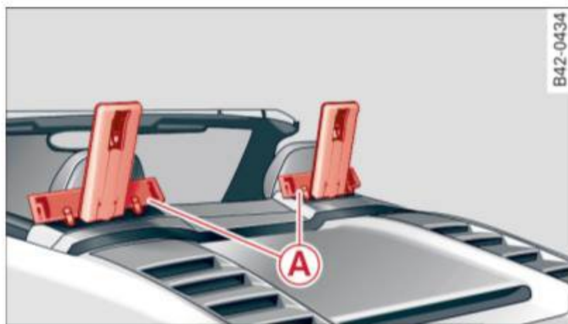
Fig. 107 Deployed rollbar with convertible top frame facing upward
