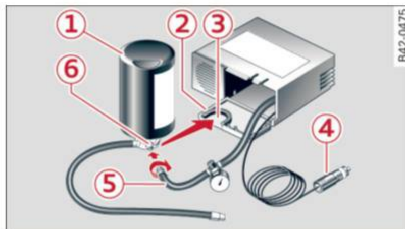
Fig. 156 Parts of the Tire Mobility System
