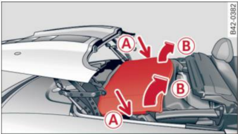
Fig. 43 Convertible top storage bay: lifting the convertible top out
