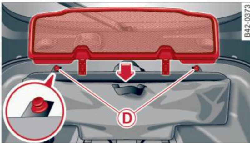
Fig. 34 Luggage compartment: storing the wind deflector
