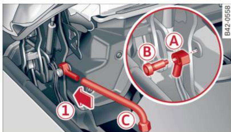
Fig. 45 Convertible top storage bay: installing the driver
