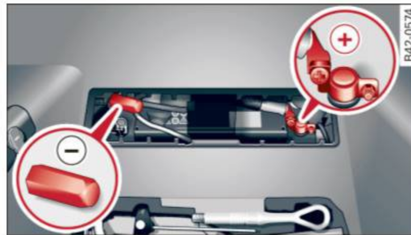
Fig. 163 Luggage compartment: connectors for a charger and jump start cables
