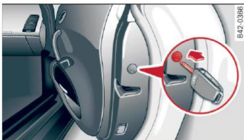
Fig. 26 Passenger's door: emergency release
