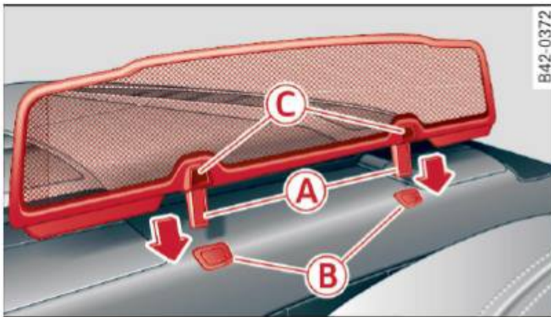
Fig. 33 Installing the wind deflector
