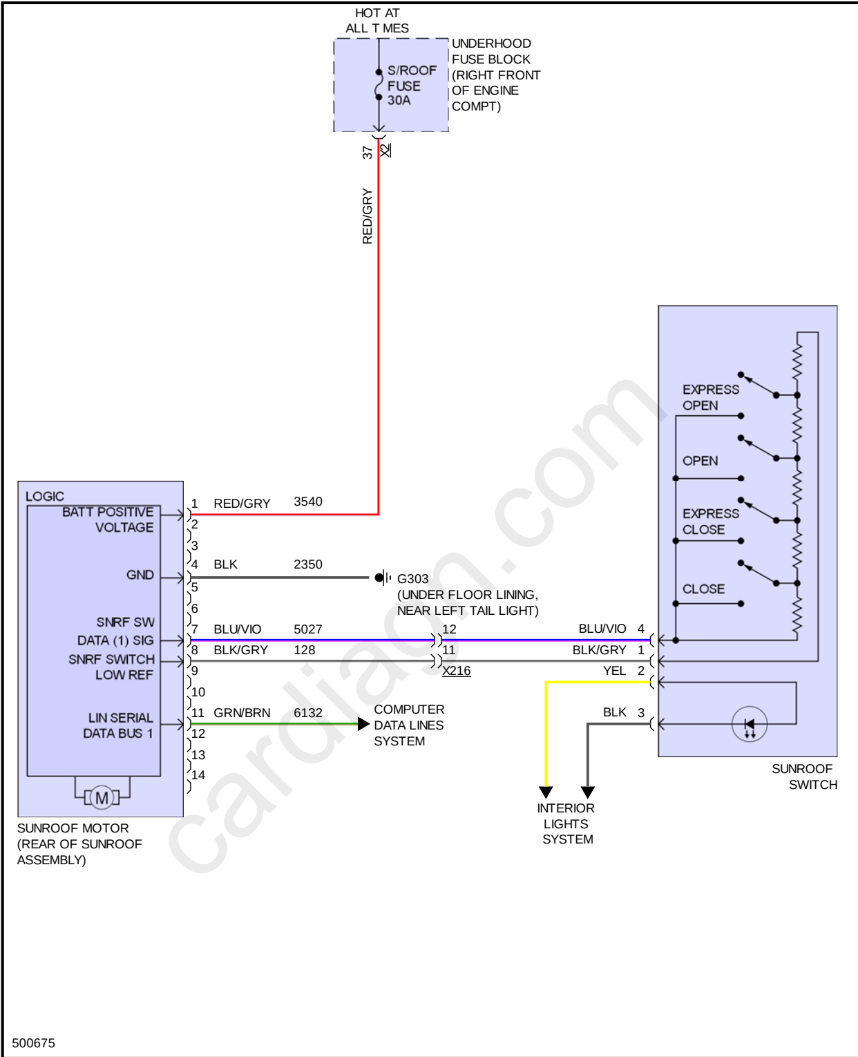
Fig 3: Sunroof Circuit
