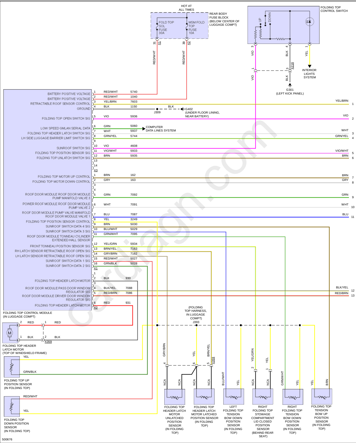
Fig 1: Electric Folding Sunroof Circuit (1 of 2)
