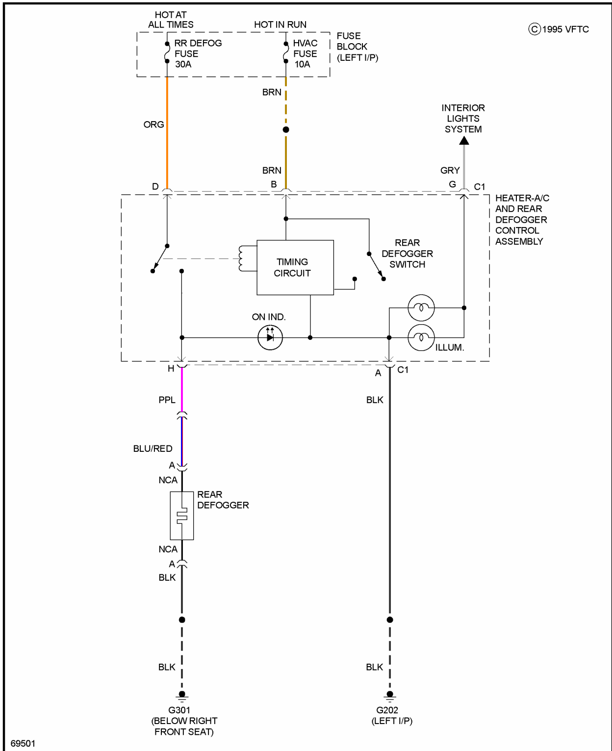
Fig. 9: Defogger Circuit
