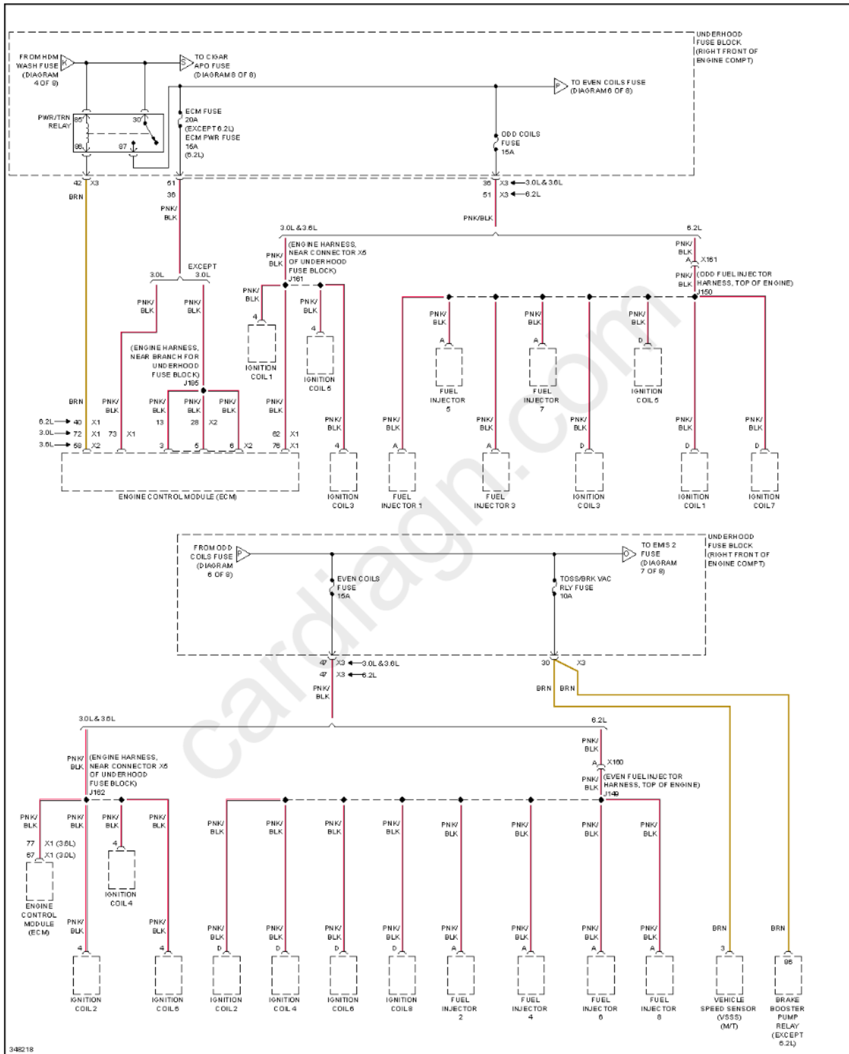
Fig. 78: Power Distribution Circuit (6 of 8)
