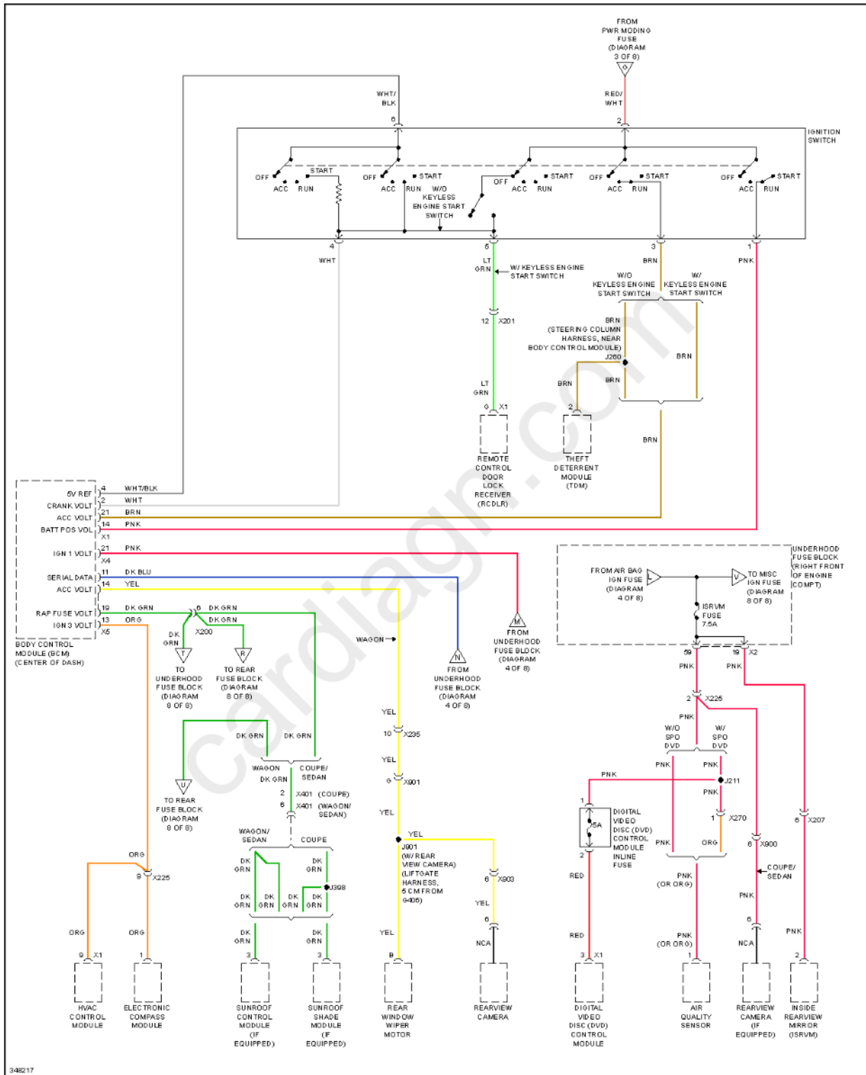
Fig. 77: Power Distribution Circuit (5 of 8)
