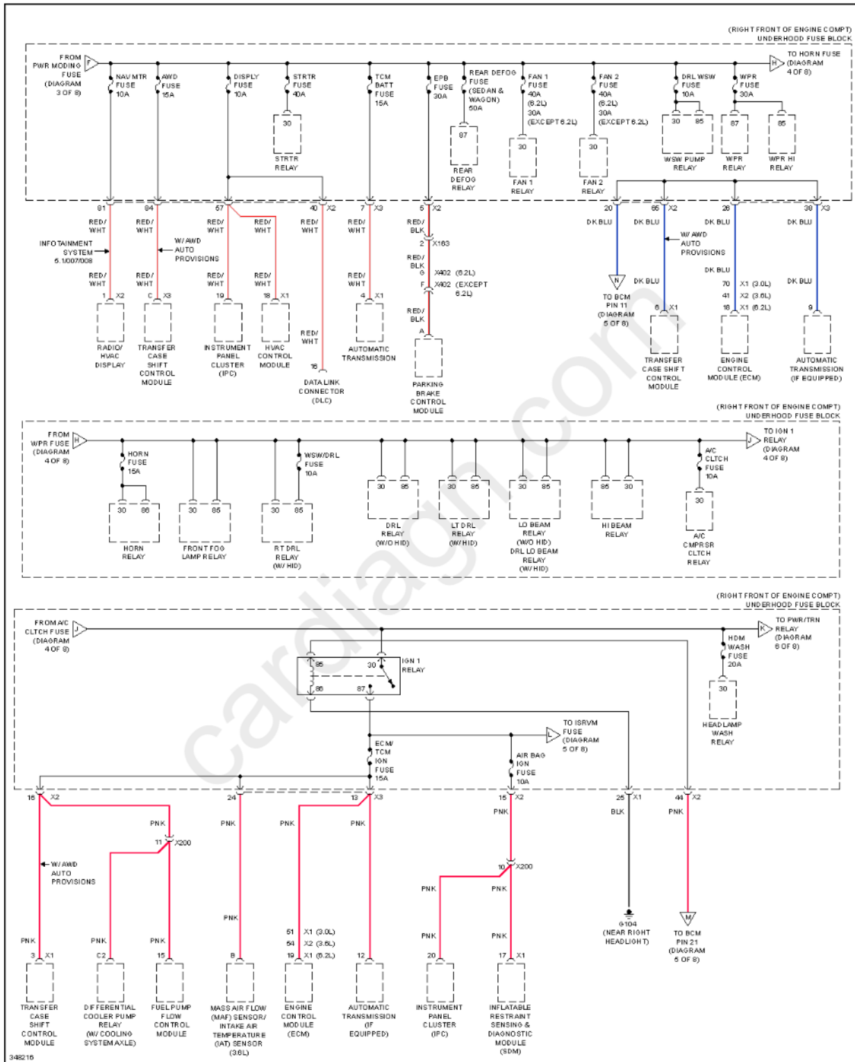
Fig. 76: Power Distribution Circuit (4 of 8)
