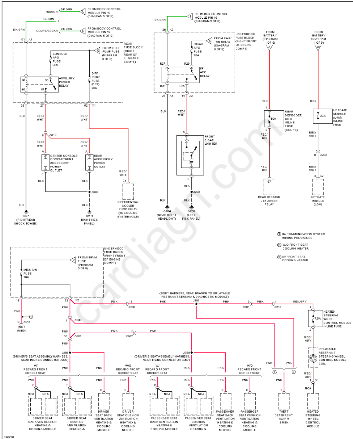
Fig. 80: Power Distribution Circuit (8 of 8)
