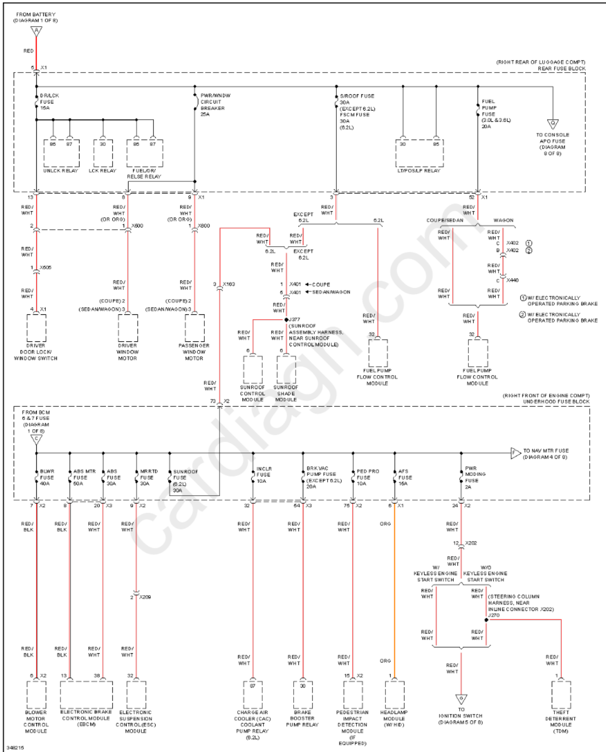
Fig. 75: Power Distribution Circuit (3 of 8)
