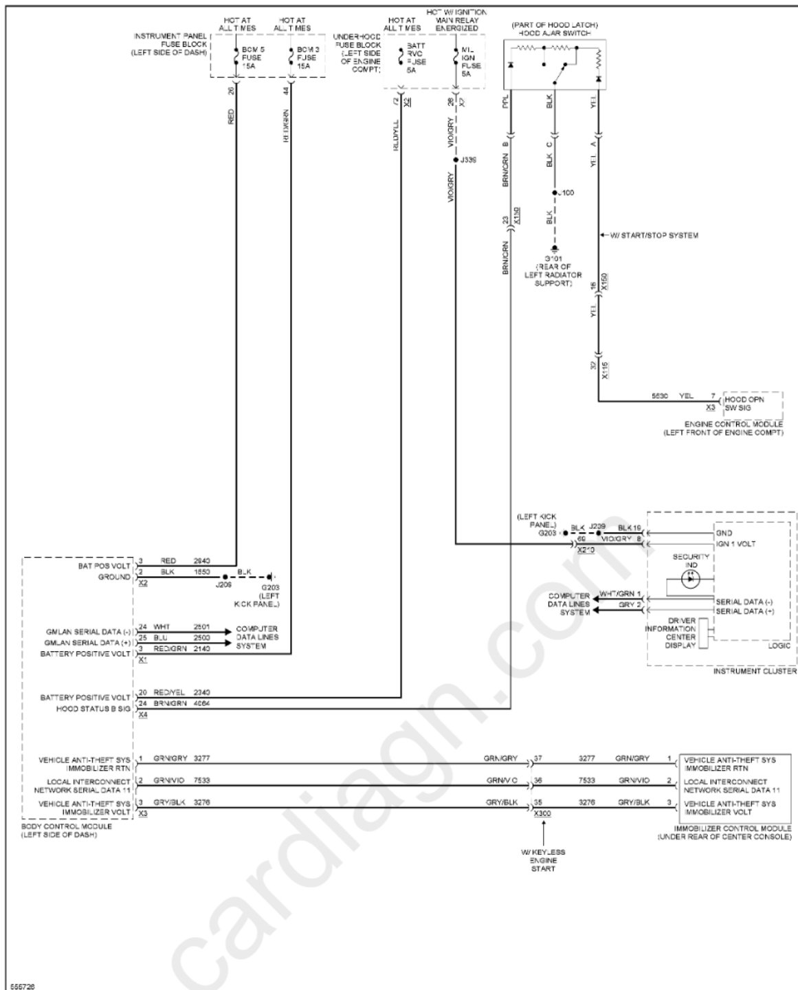
Fig. 18: Pass-Key Circuit
