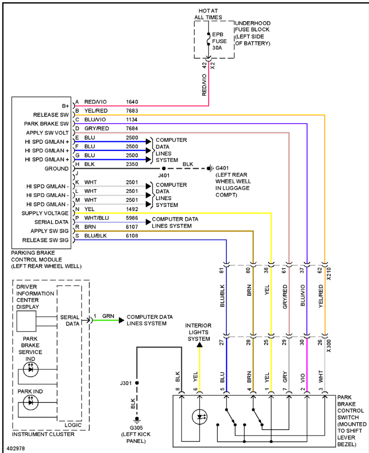
Fig. 122: Park Brake System Circuit
