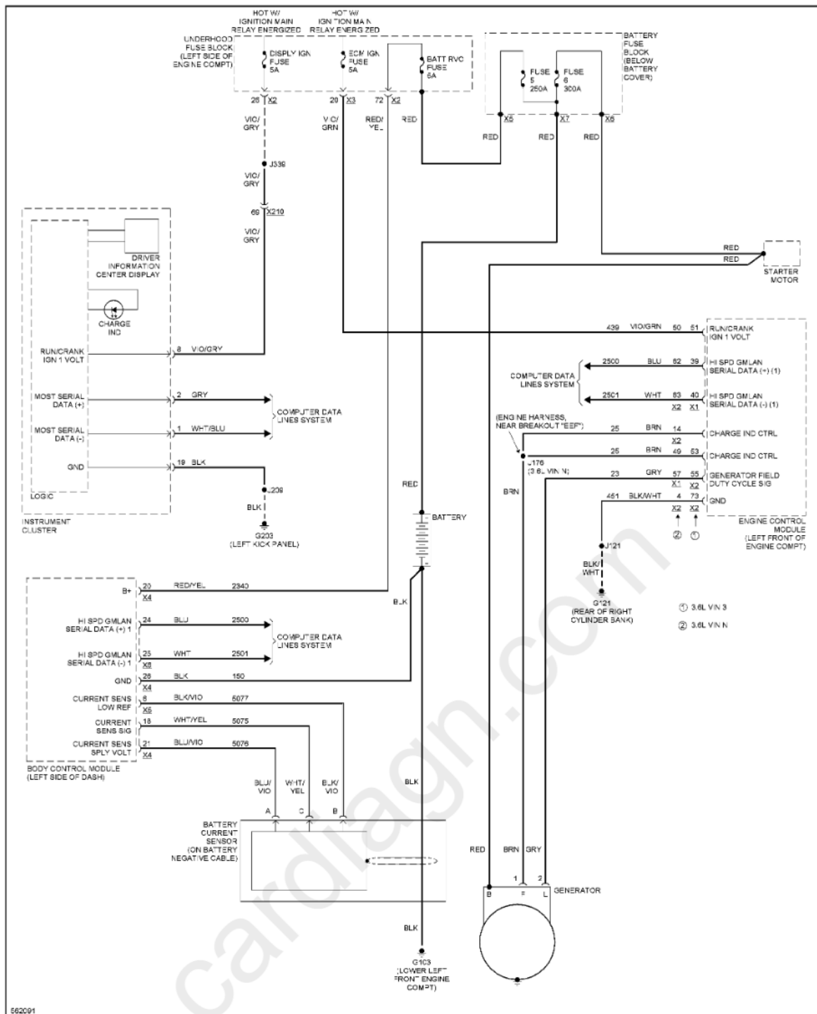
Fig. 119: Charging Circuit, W/O Start-Stop System
