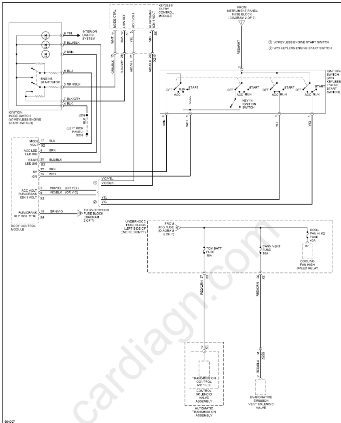
Fig. 89: Power Distribution Circuit (6 of 7)
