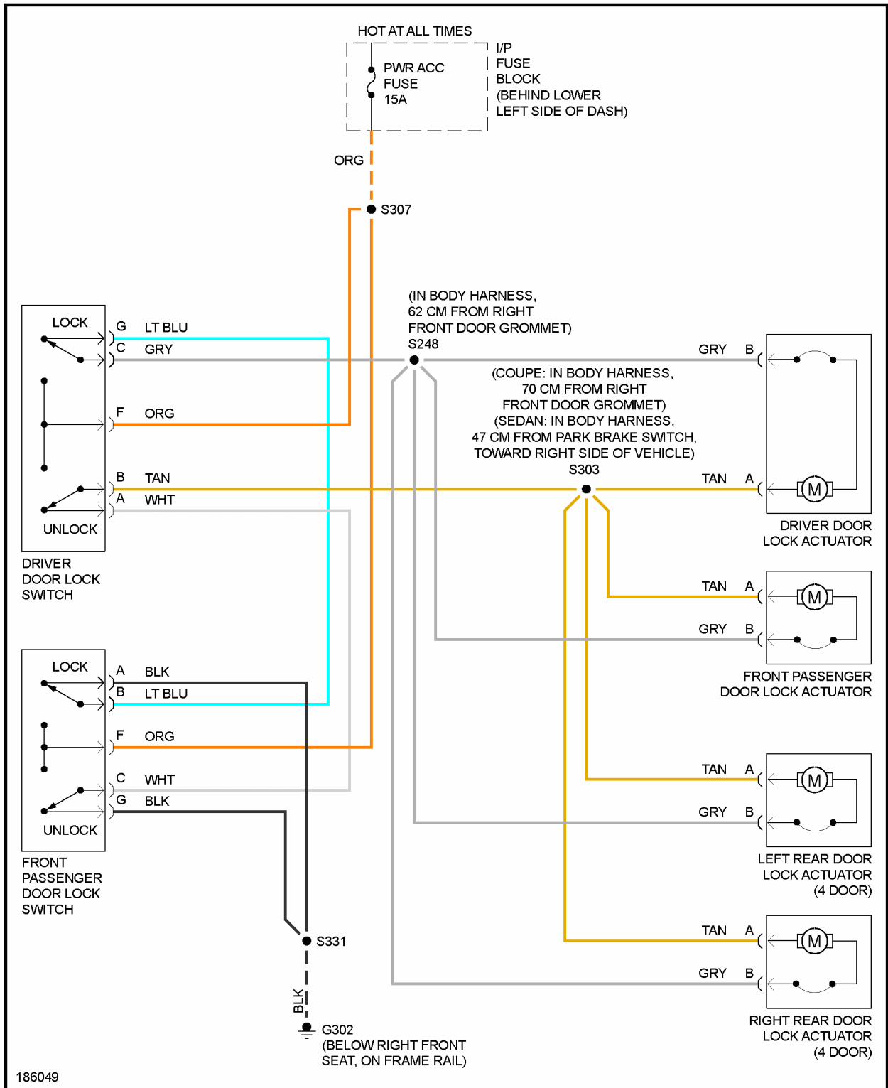
Fig. 25: Power Door Locks Circuit, W/O Keyless Entry
