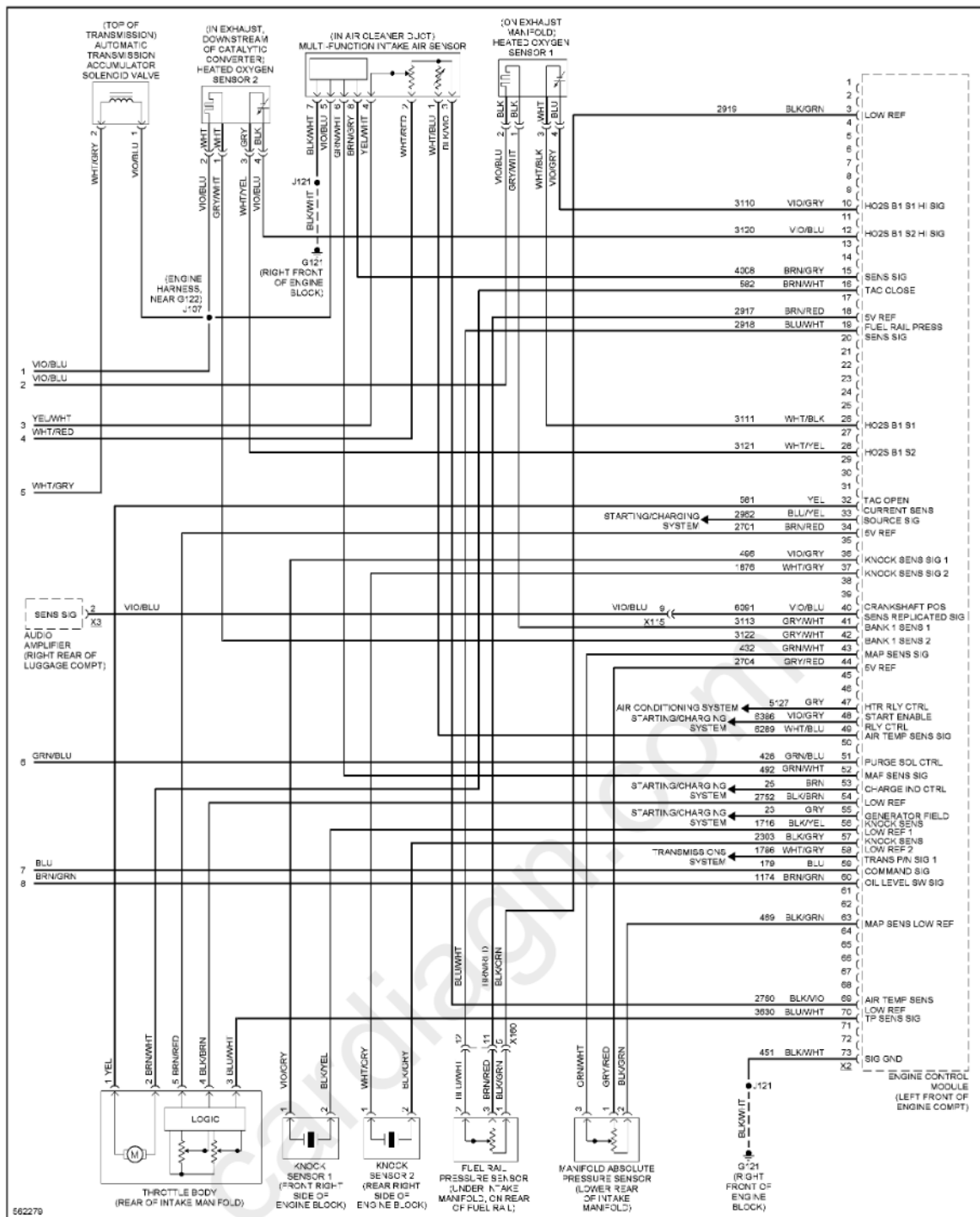
Fig. 40: 2.5L VIN A, Engine Performance Circuit (6 of 6)
