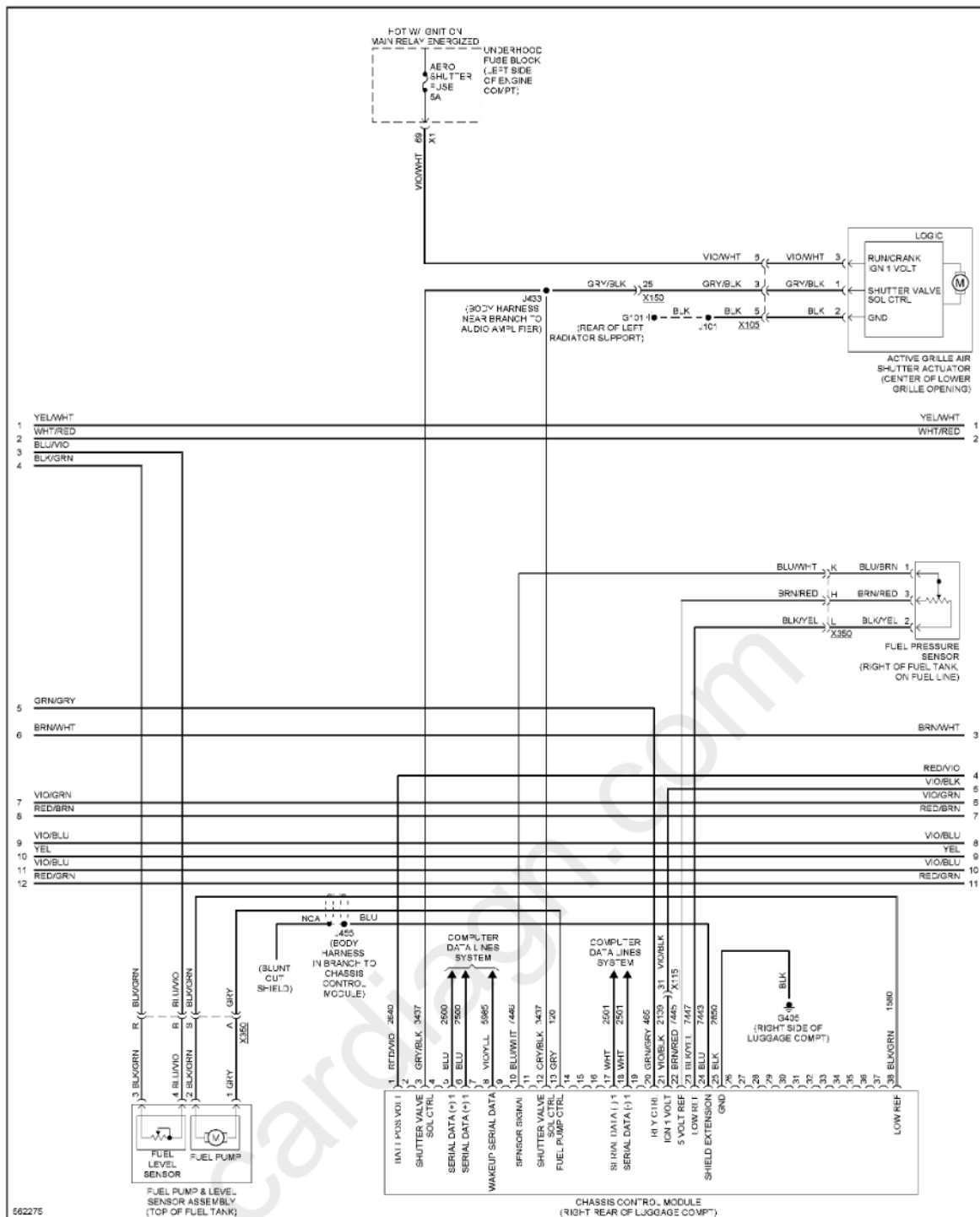
Fig. 36: 2.5L VIN A, Engine Performance Circuit (2 of 6)
