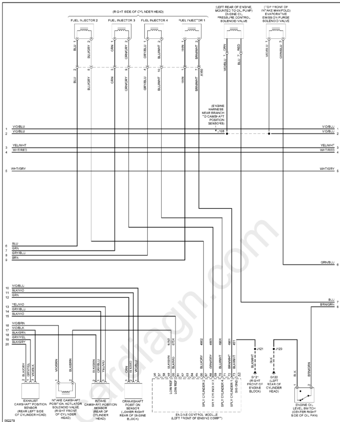
Fig. 39: 2.5L VIN A, Engine Performance Circuit (5 of 6)
