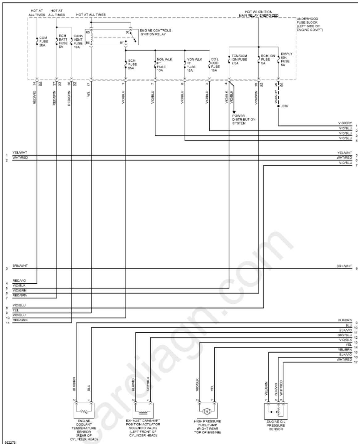
Fig. 37: 2.5L VIN A, Engine Performance Circuit (3 of 6)
