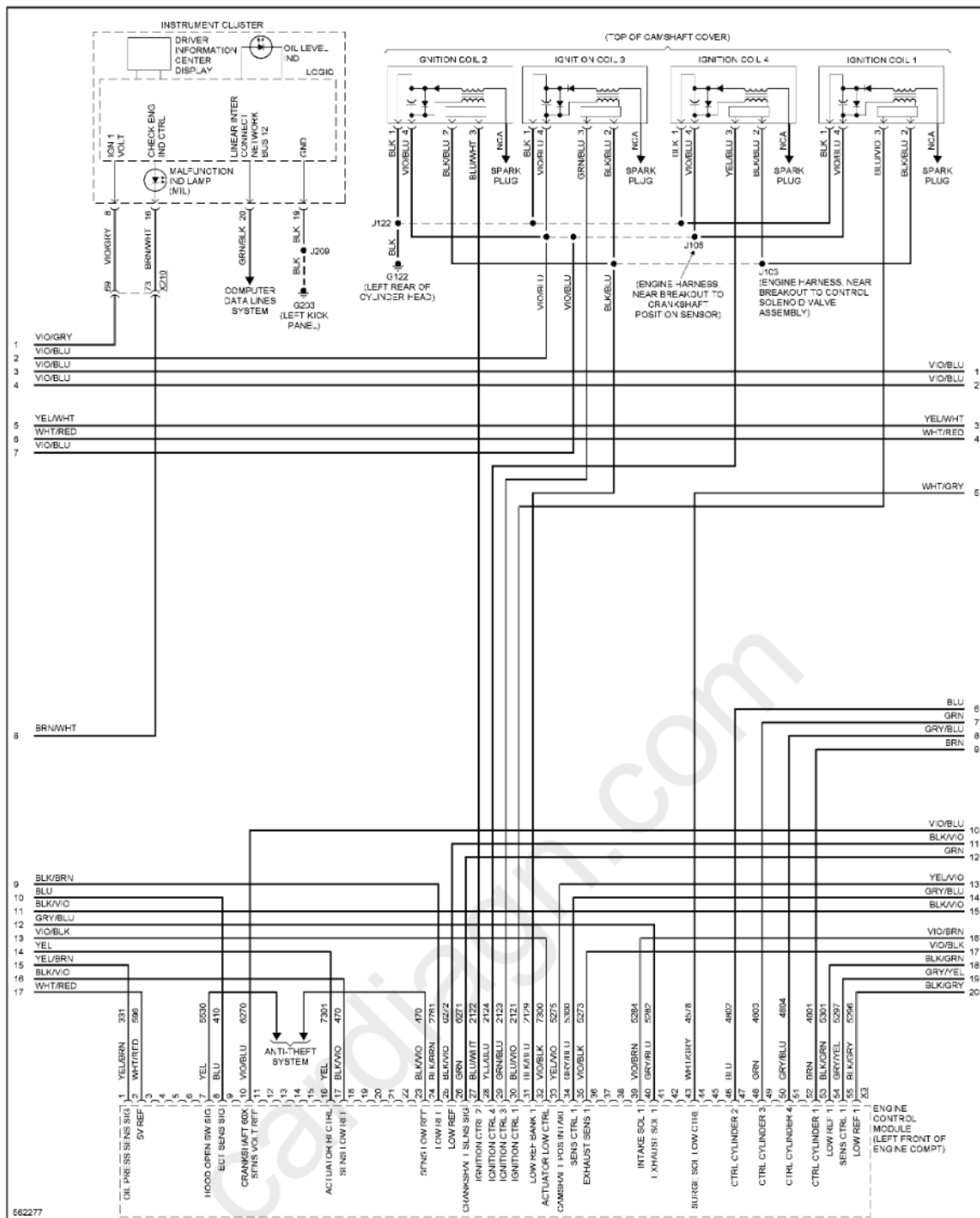
Fig. 38: 2.5L VIN A, Engine Performance Circuit (4 of 6)
