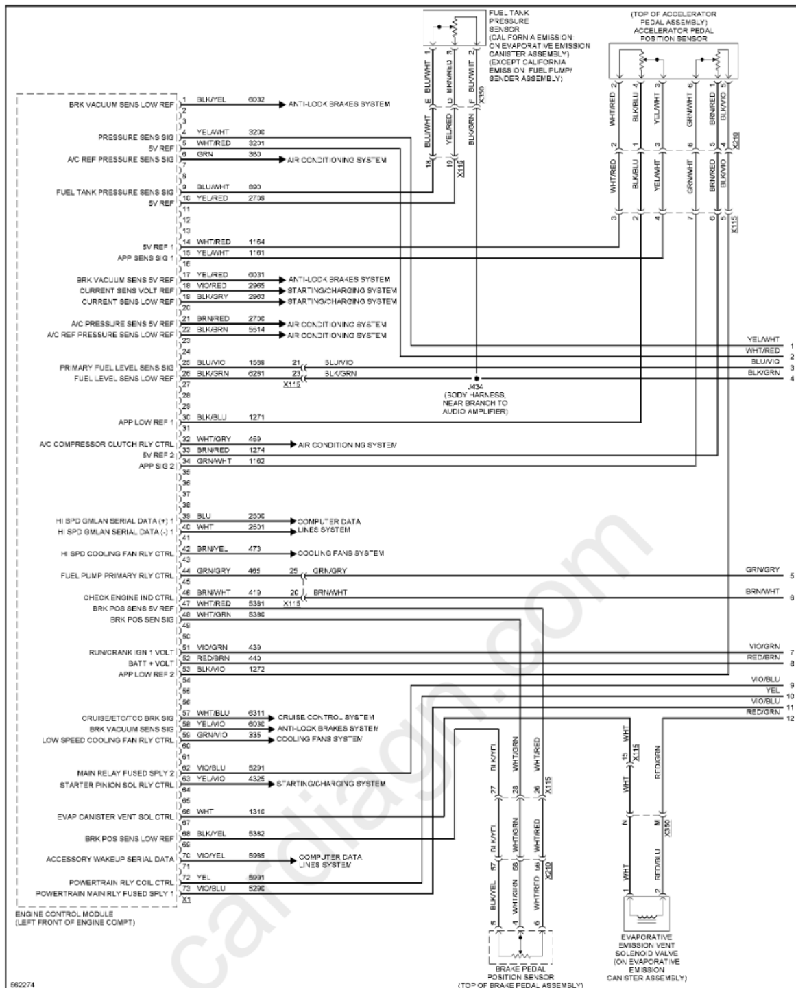
Fig. 35: 2.5L VIN A, Engine Performance Circuit (1 of 6)
