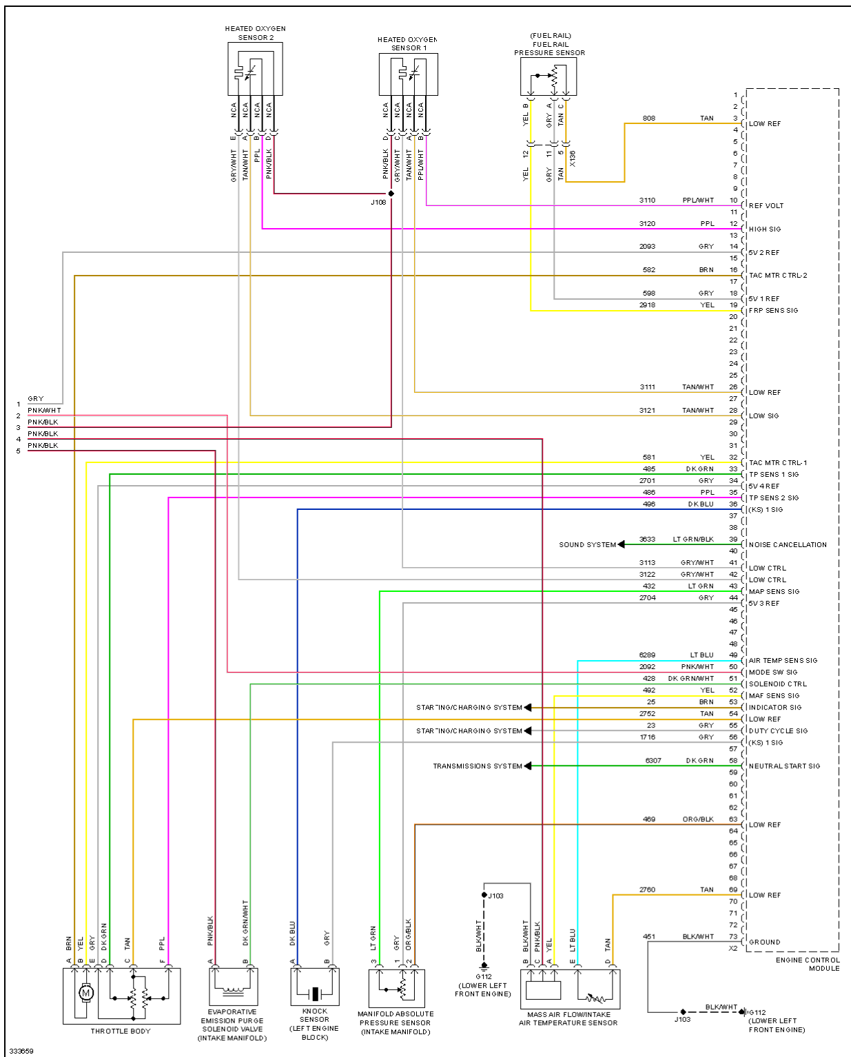
Fig. 23: 2.4L VIN W, Engine Performance Circuit (5 of 5)
