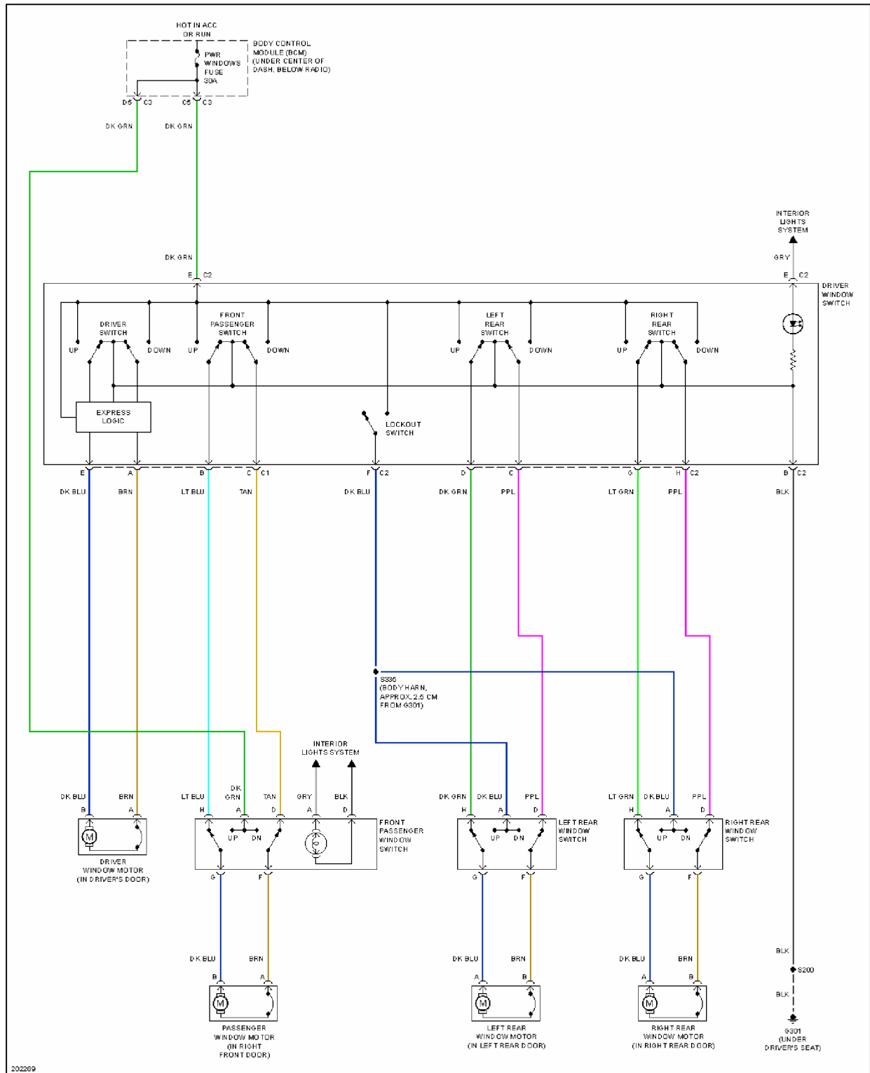
Fig. 49: Power Windows Circuit, Sedan
