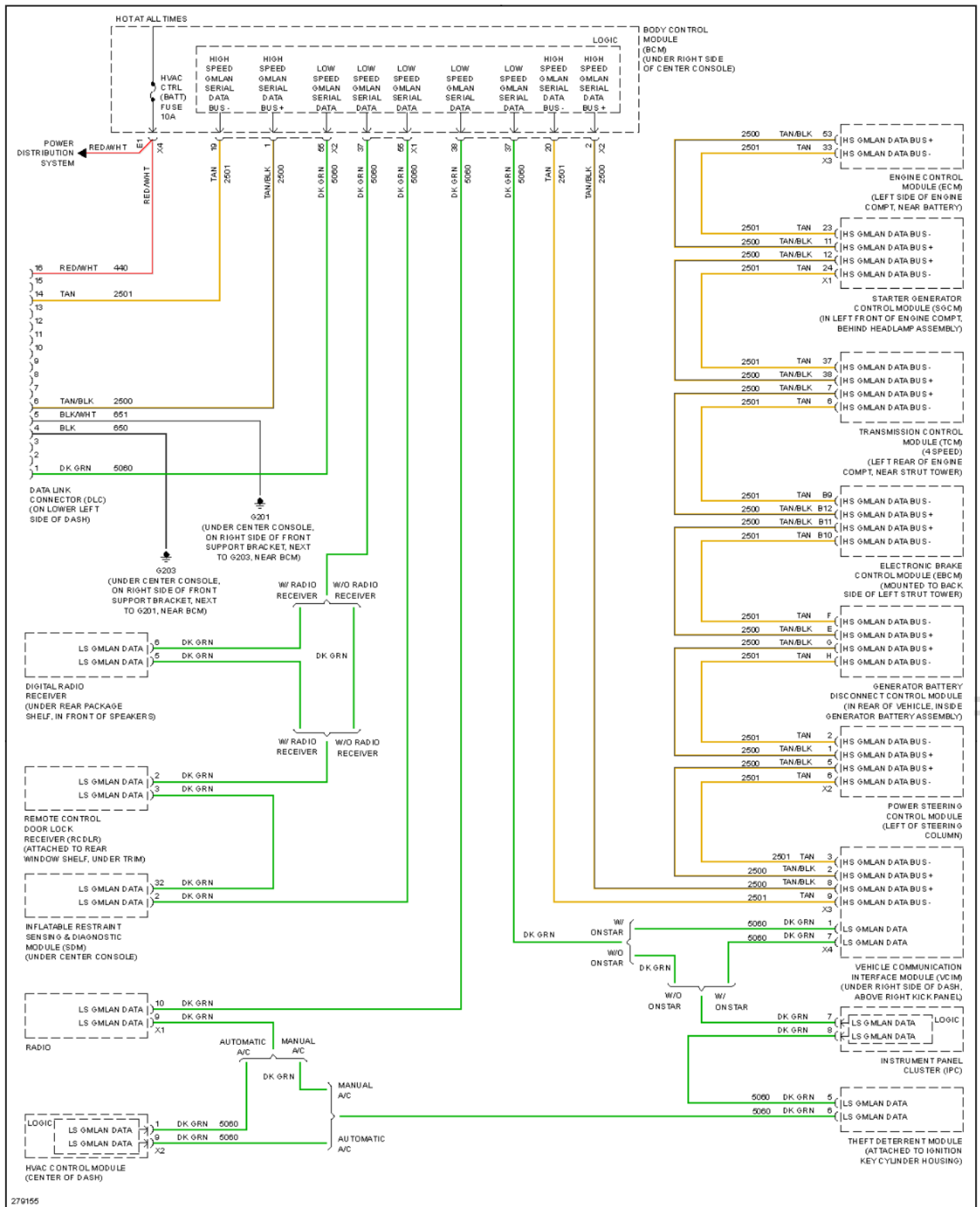
Fig. 16: Computer Data Lines Circuit, Hybrid
