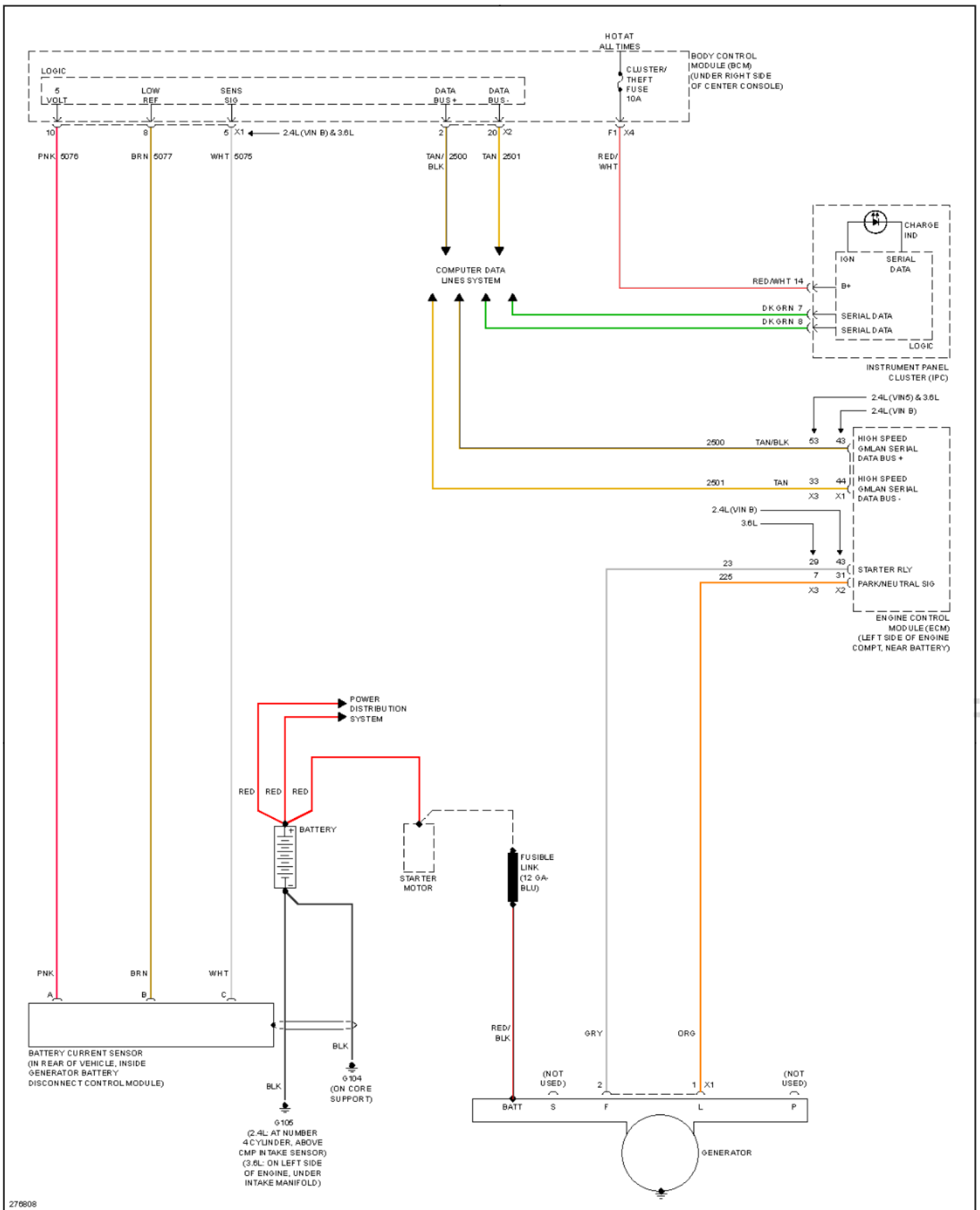
Fig. 77: Charging Circuit
