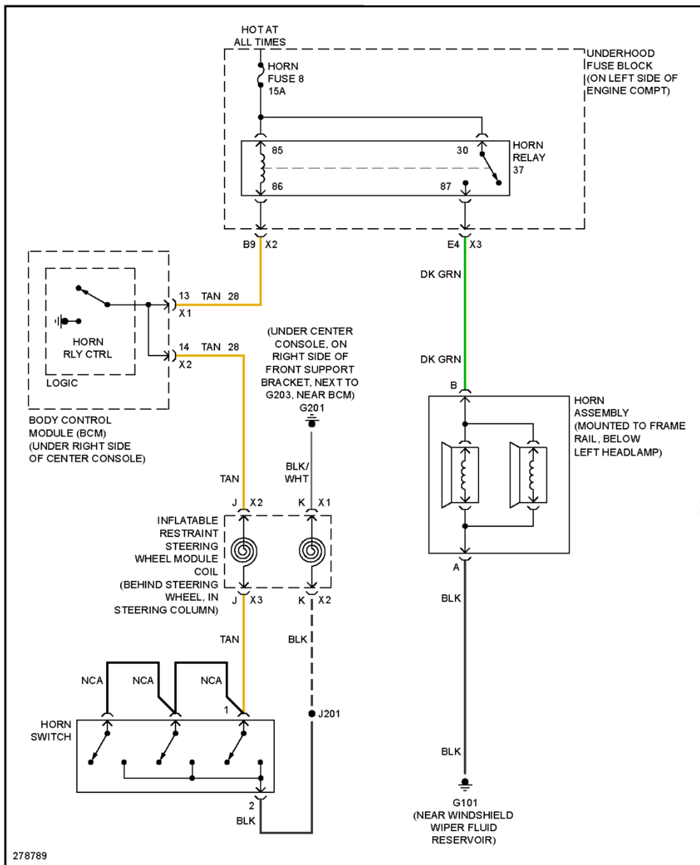
Fig. 50: Horn Circuit
