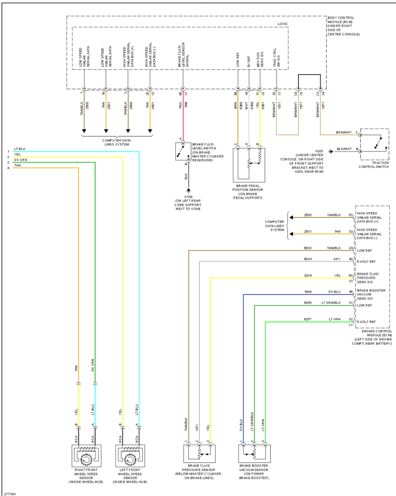
Fig. 9: Anti-lock Brakes Circuit, Hybrid (2 of 2)
