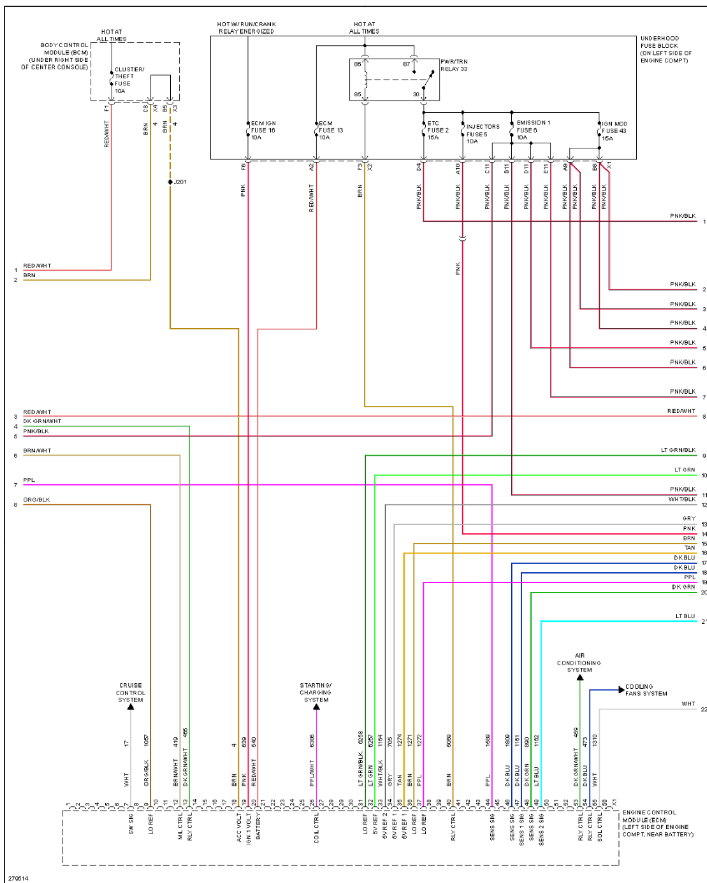
Fig. 23: 2.4L VIN 5, Engine Controls Circuit (2 of 4)
