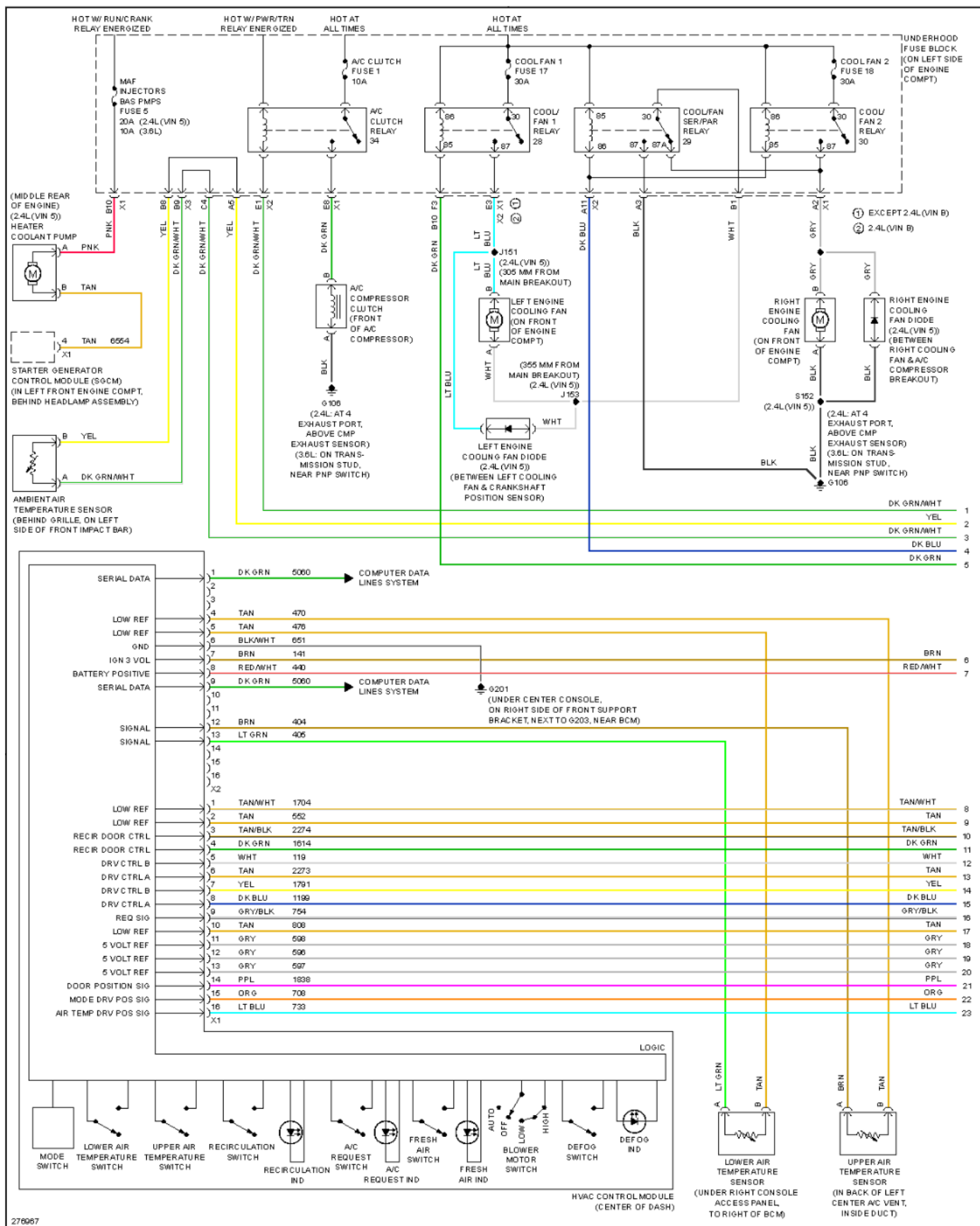
Fig. 1: Automatic A/C Circuit (1 of 2)
