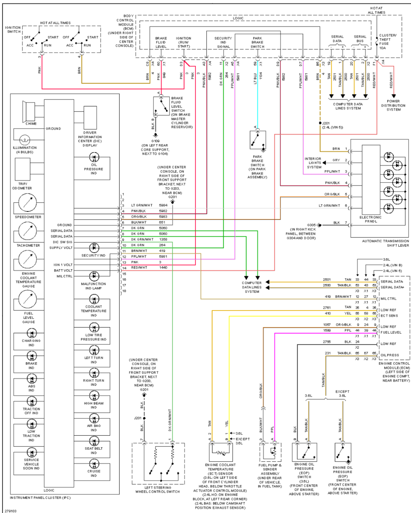
Fig. 51: Instrument Cluster Circuit
