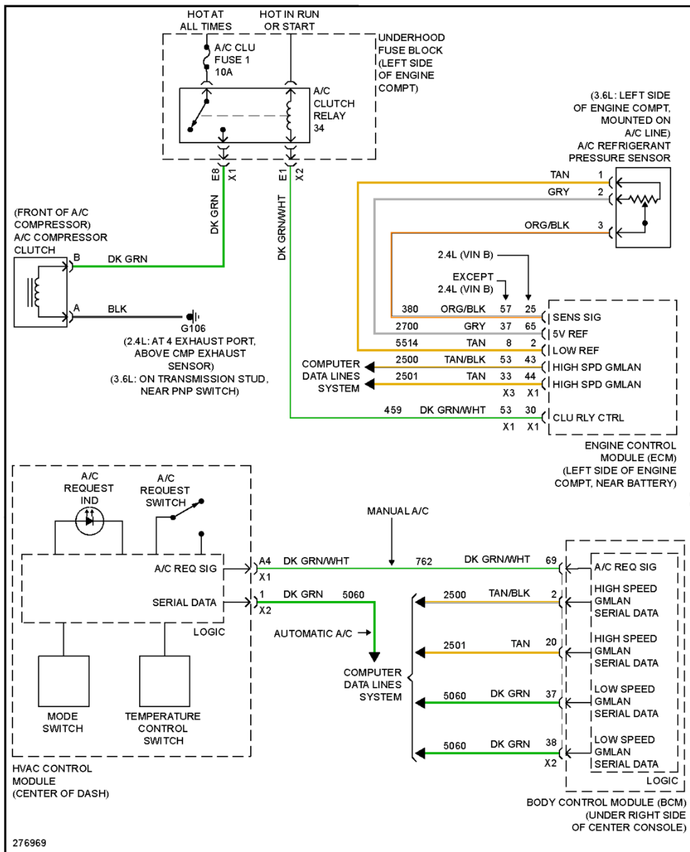
Fig. 3: Compressor Circuit
