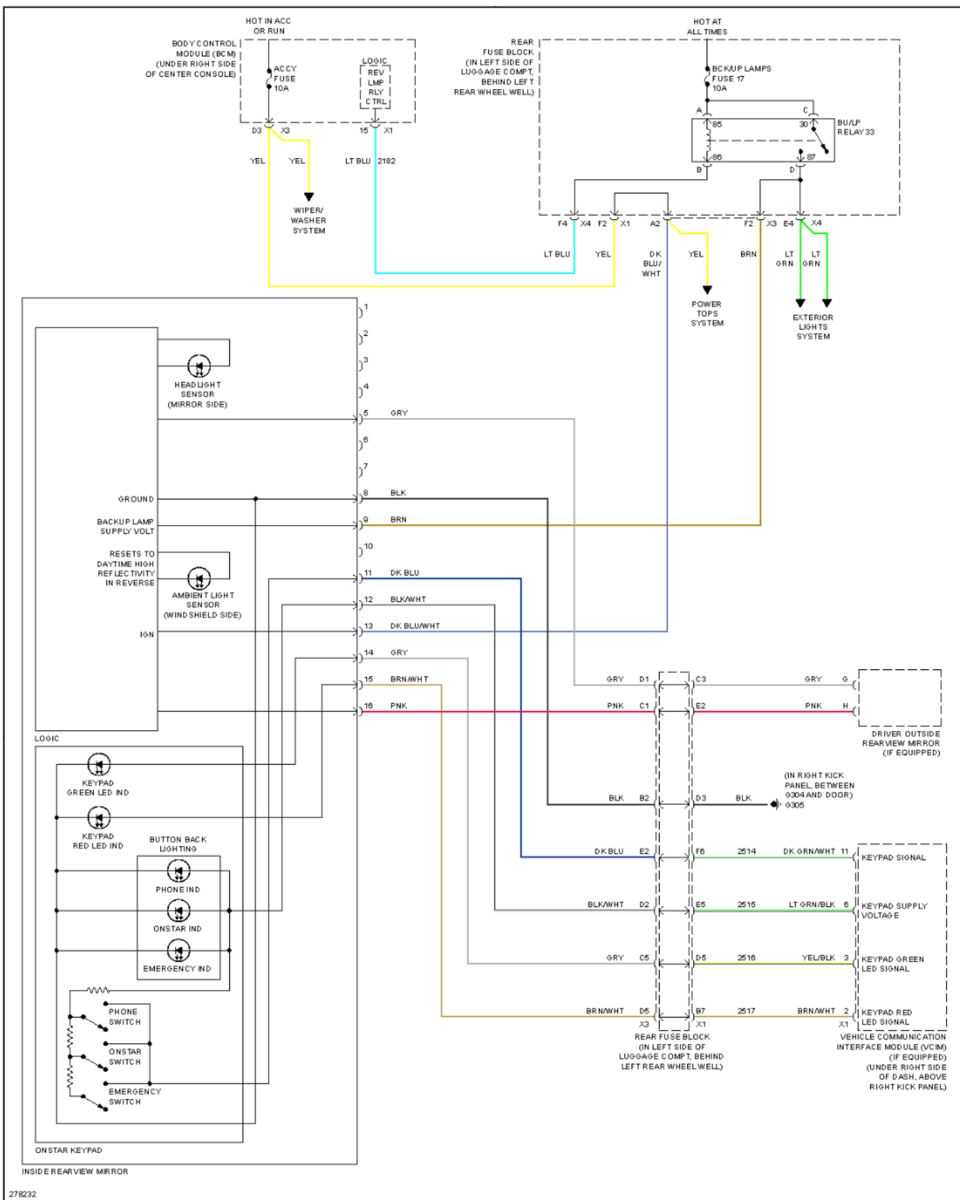
Fig. 59: Automatic Day/Night Mirror Circuit
