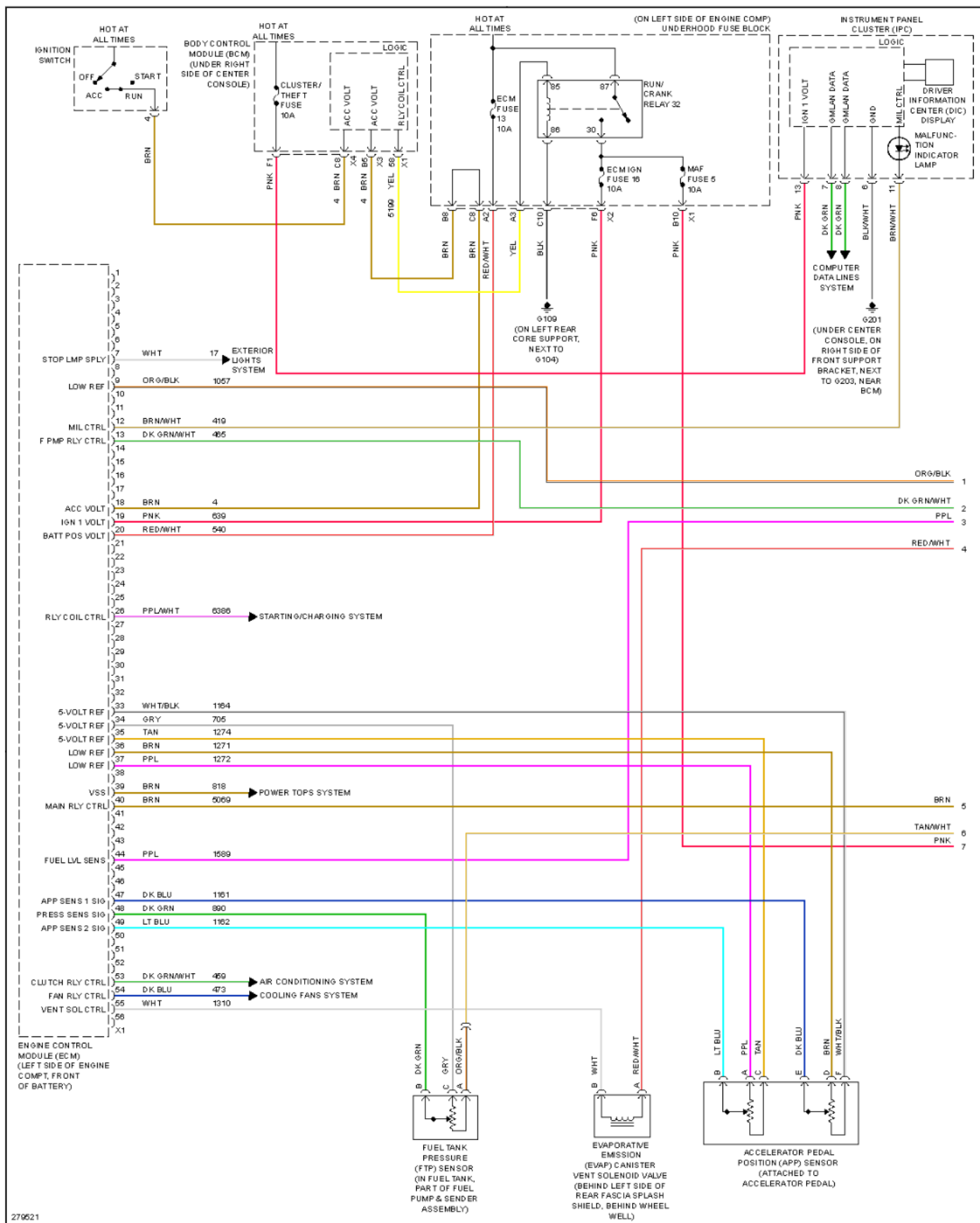
Fig. 37: 3.6L VIN 7, Engine Performance Circuit (1 of 6)
