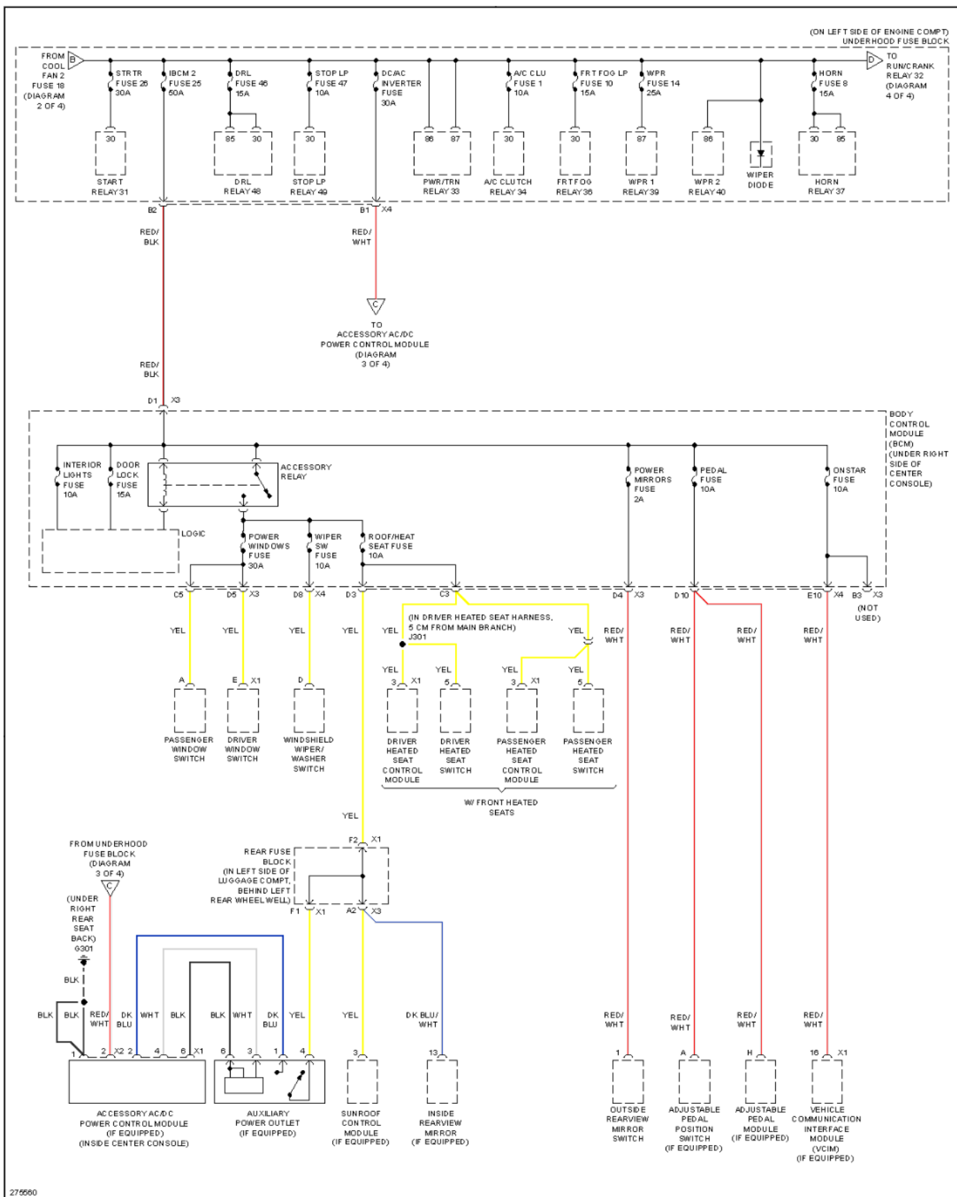
Fig. 56: Power Distribution Circuit (3 of 4)
