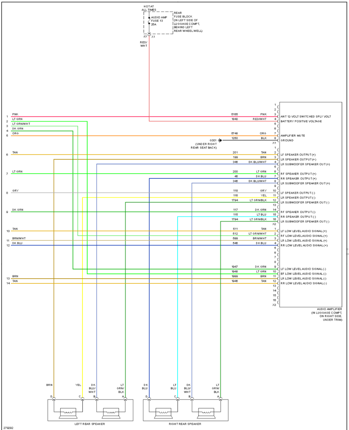
Fig. 72: Radio Circuit, Enhanced (3 of 3)
