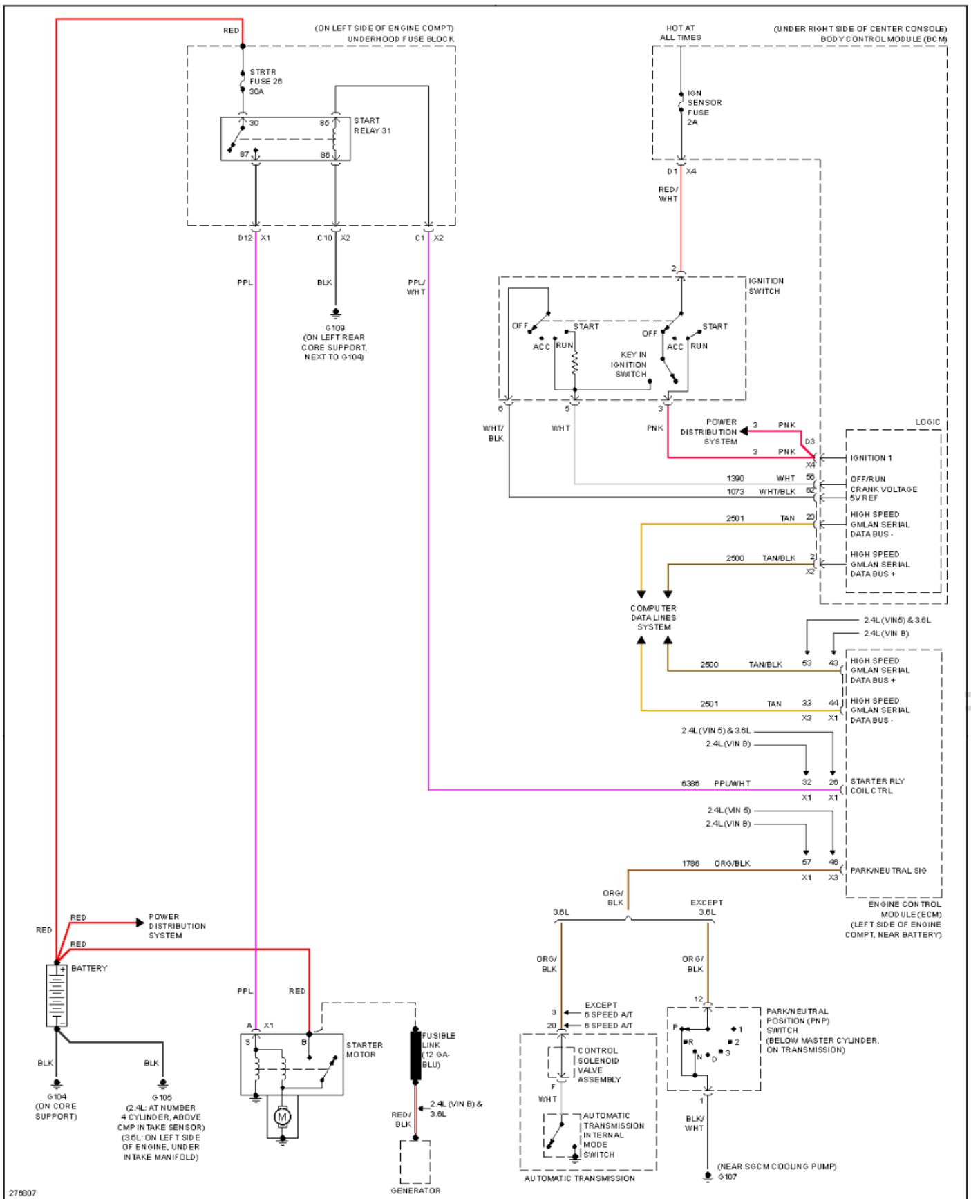
Fig. 78: Starting Circuit
