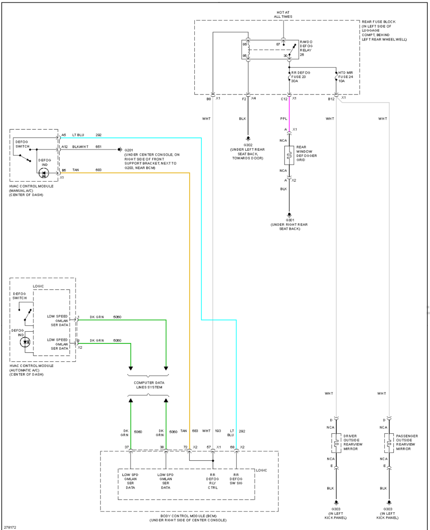
Fig. 20: Defoggers Circuit
