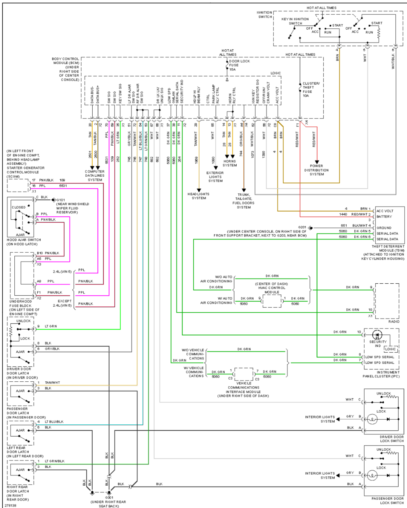
Fig. 10: Anti-theft Circuit
