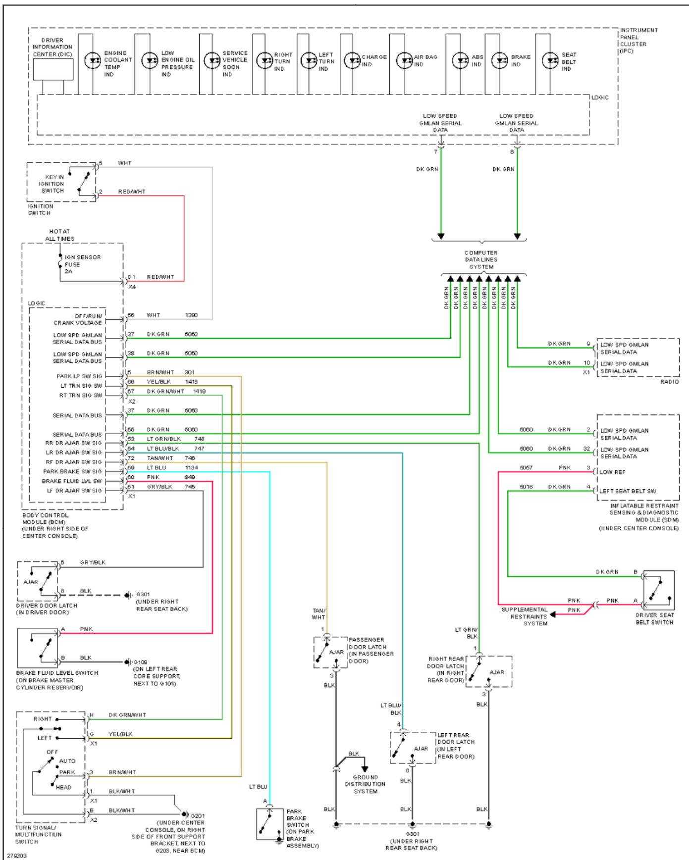
Fig. 91: Warning Systems Circuit
