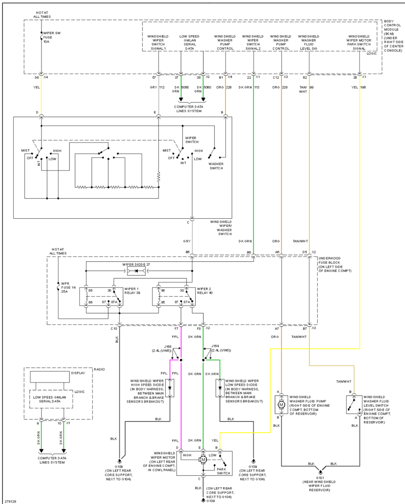
Fig. 92: Wiper/Washer Circuit
