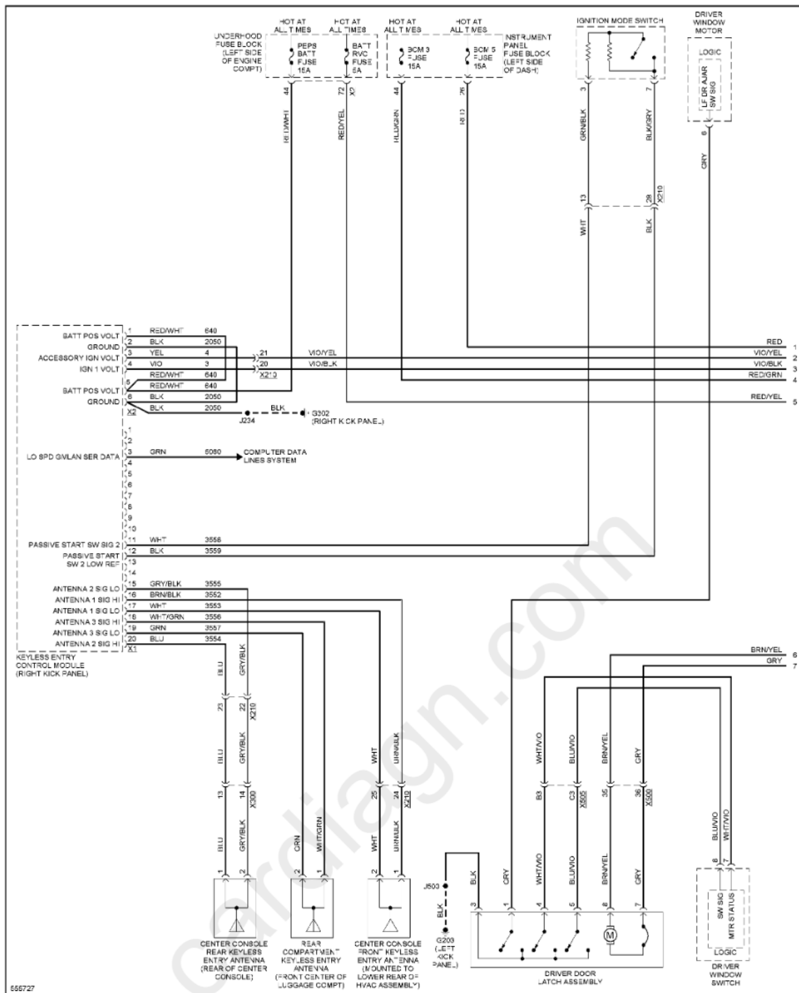
Fig. 11: Forced Entry Circuit, W/ Passive Keyless Entry (1 of 4)
