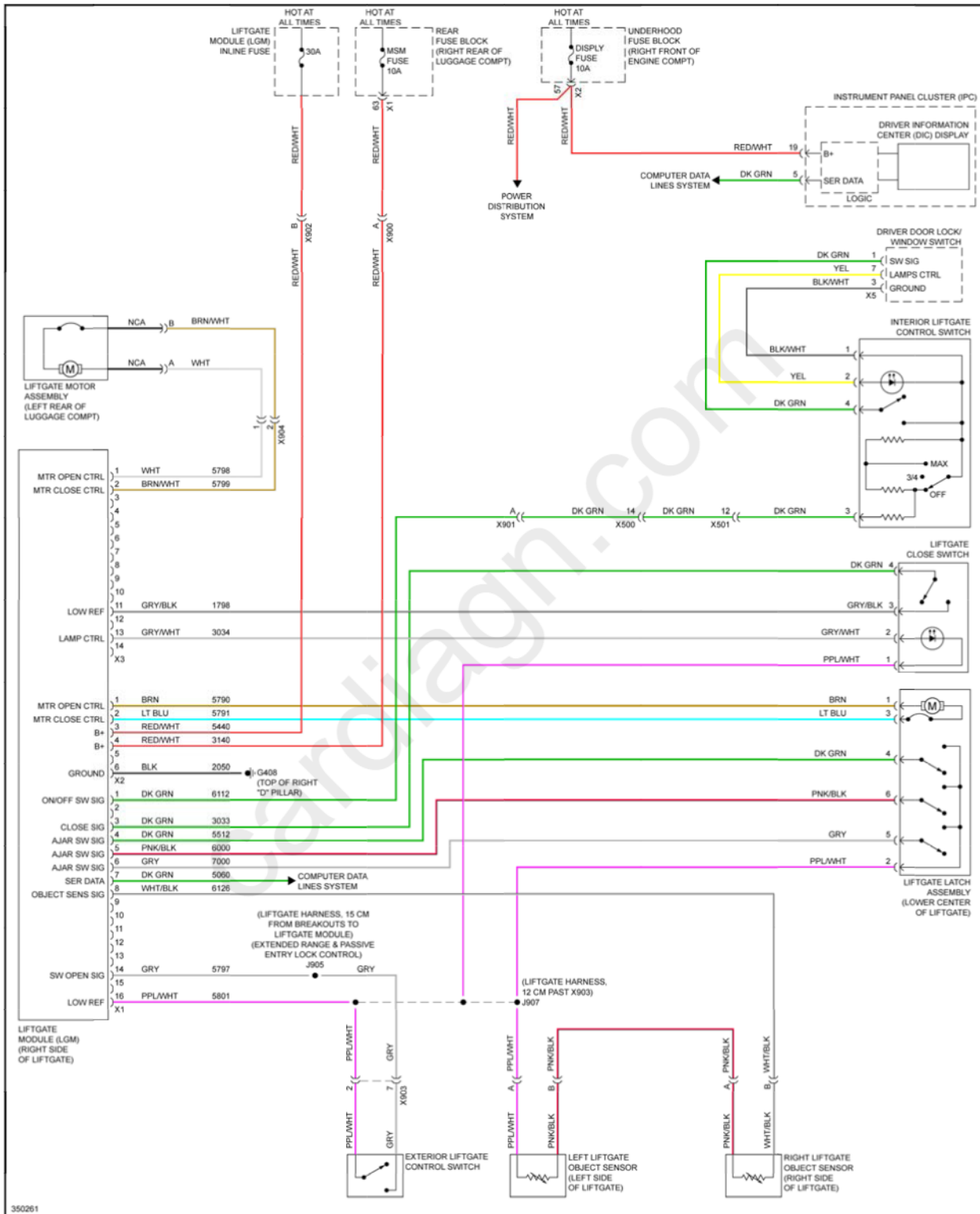
Fig. 118: Liftgate Release Circuit
