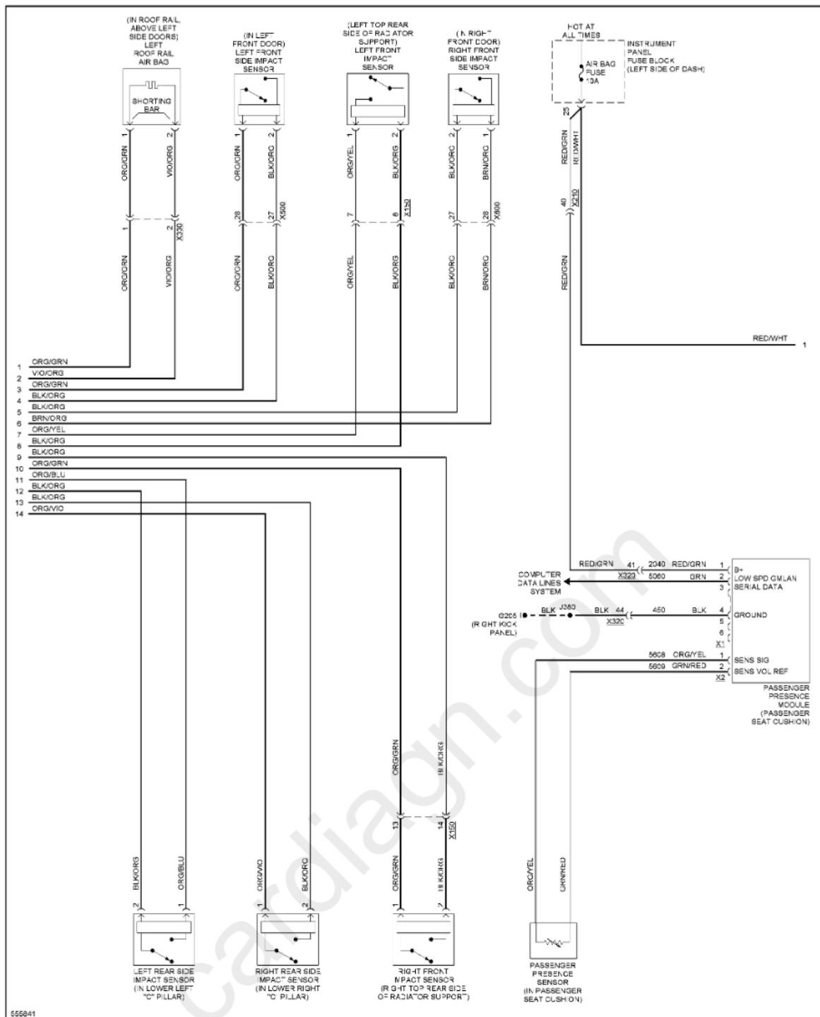
Fig. 123: Supplemental Restraints Circuit (2 of 3)
