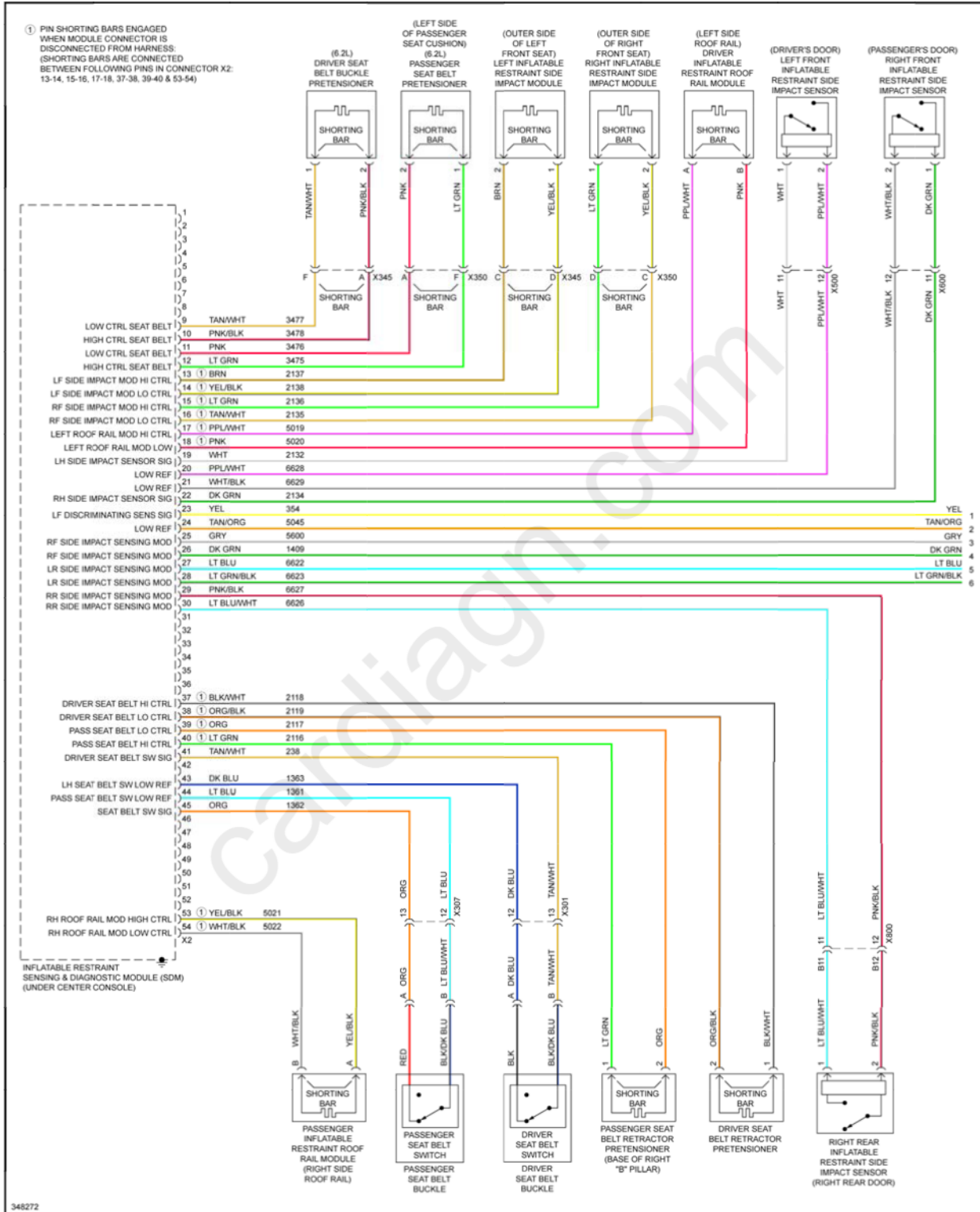
Fig. 113: Supplemental Restraints Circuit (1 of 2)
