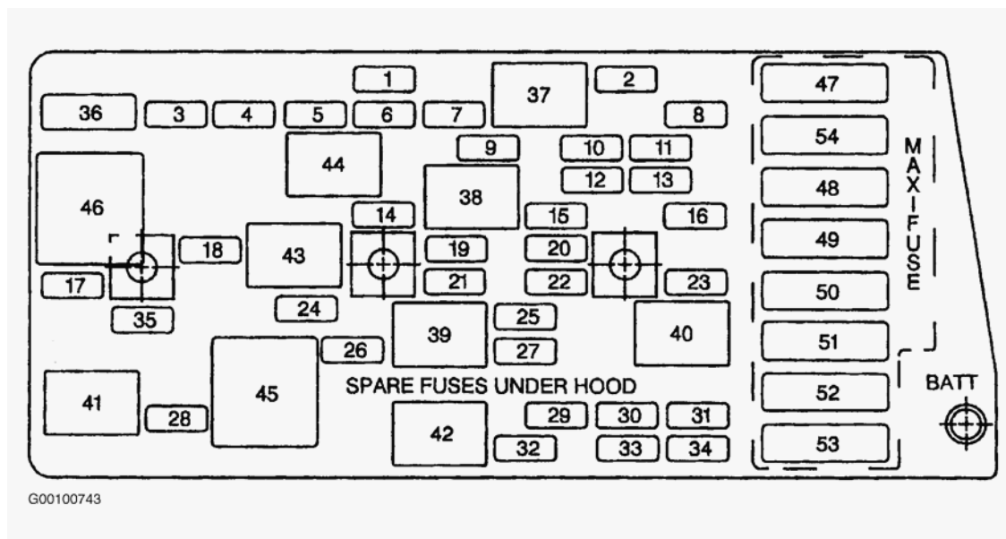
Fig. 2: Identifying Instrument Panel Fuse Block Courtesy of GENERAL MOTORS CORP.
