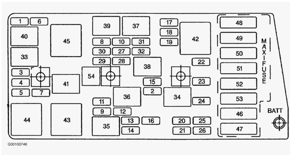
Fig. 5: Identifying Underhood Fuse Block Components Courtesy of GENERAL MOTORS CORP.
