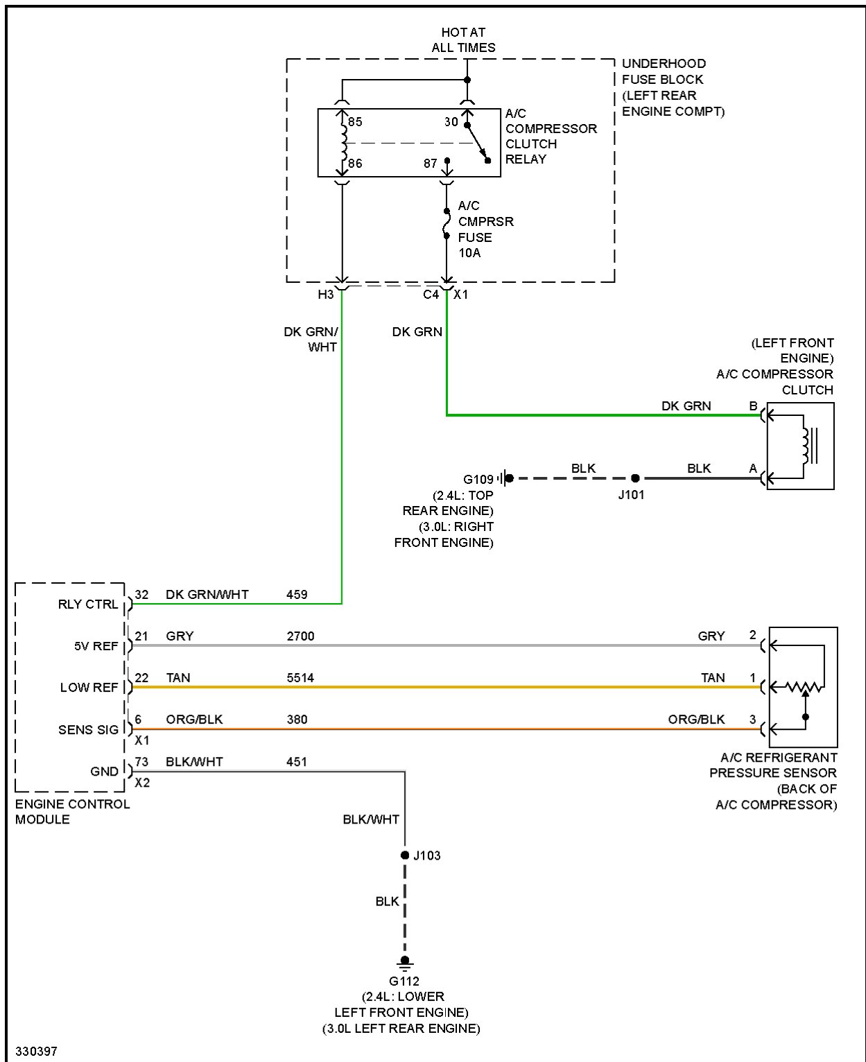
Fig. 3: Compressor Circuit
