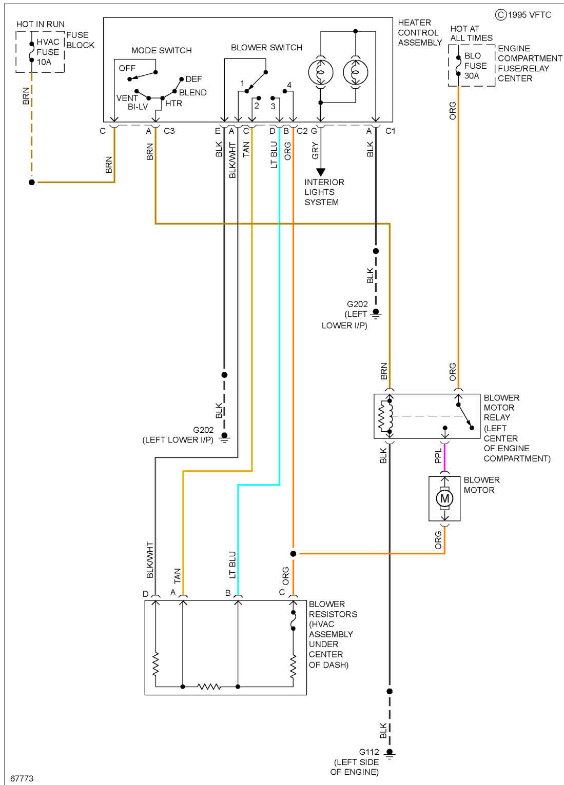
Fig. 2: Heater Circuit
