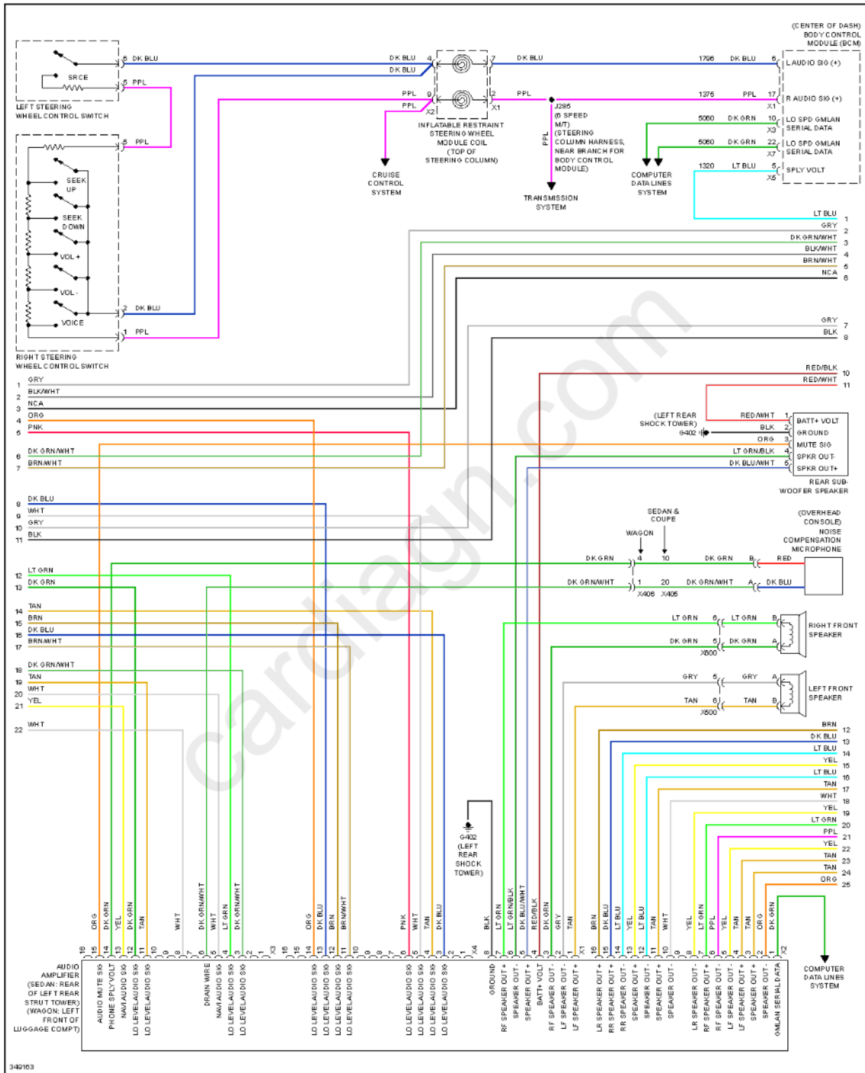
Fig. 65: Navigation Circuit, W/ Surround Amplifier (3 of 4)
