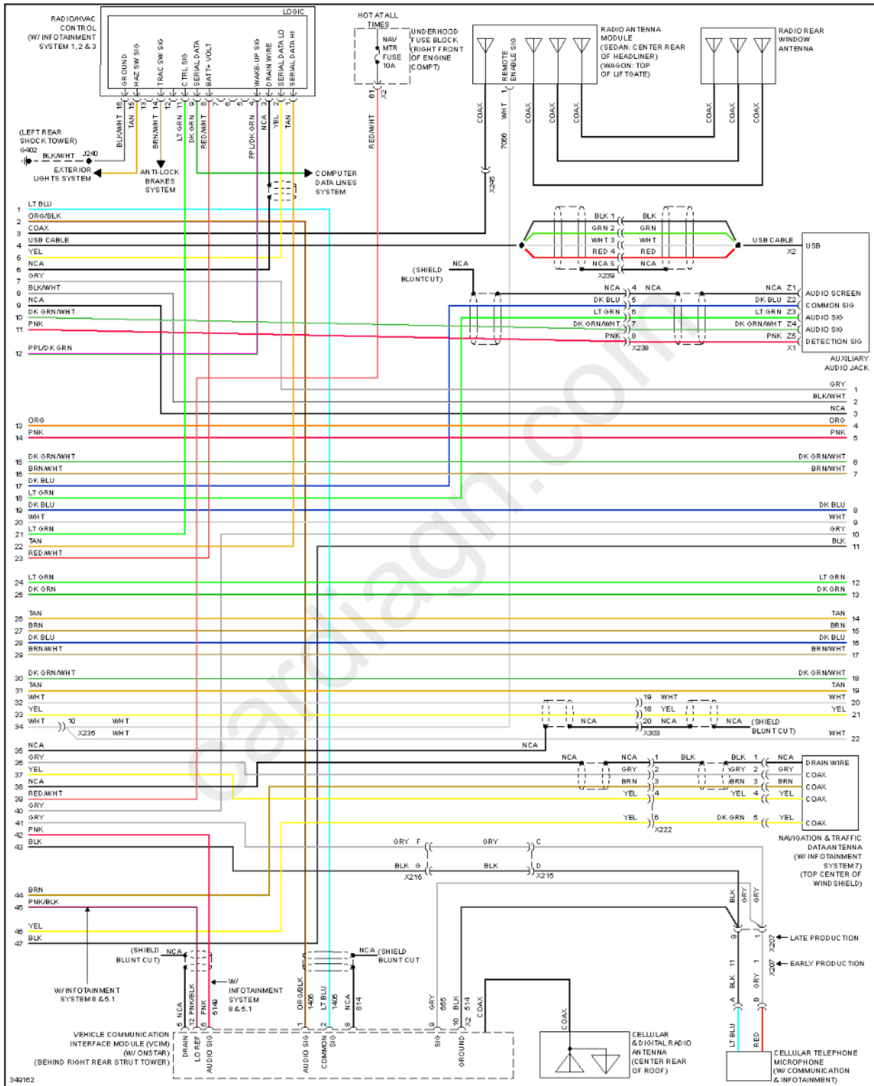
Fig. 64: Navigation Circuit, W/ Surround Amplifier (2 of 4)
