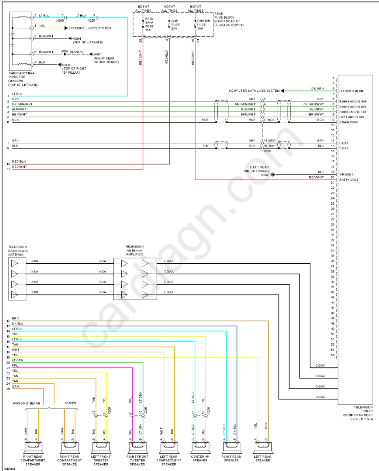
Fig. 66: Navigation Circuit, W/ Surround Amplifier (4 of 4)
