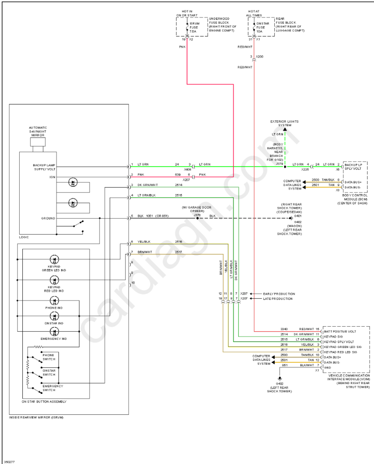
Fig. 85: Automatic Day/Night Mirror Circuit, W/ Infotainment System 1/2/3 W/O Rearview Camera
