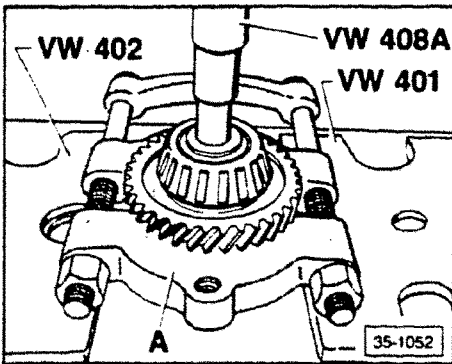
► Fig. 14 Taper roller bearing — inner race, removing
