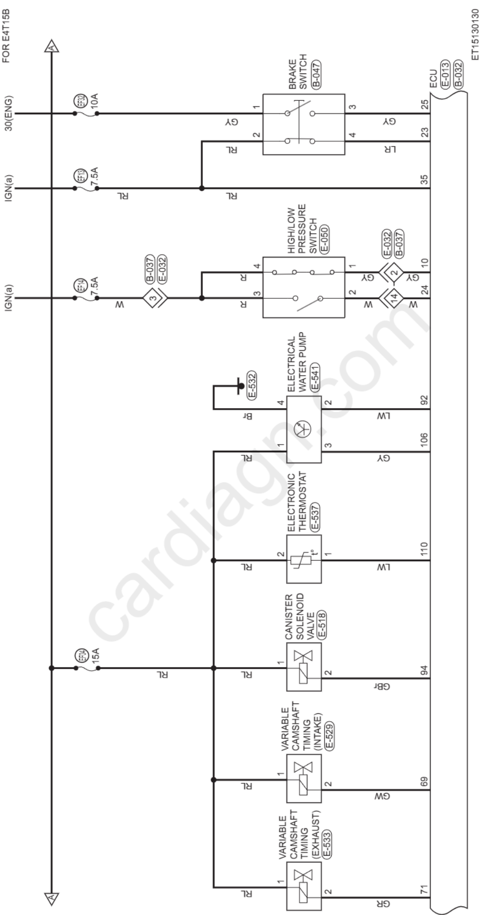
Circuit Diagram (Page 3 of 6)
