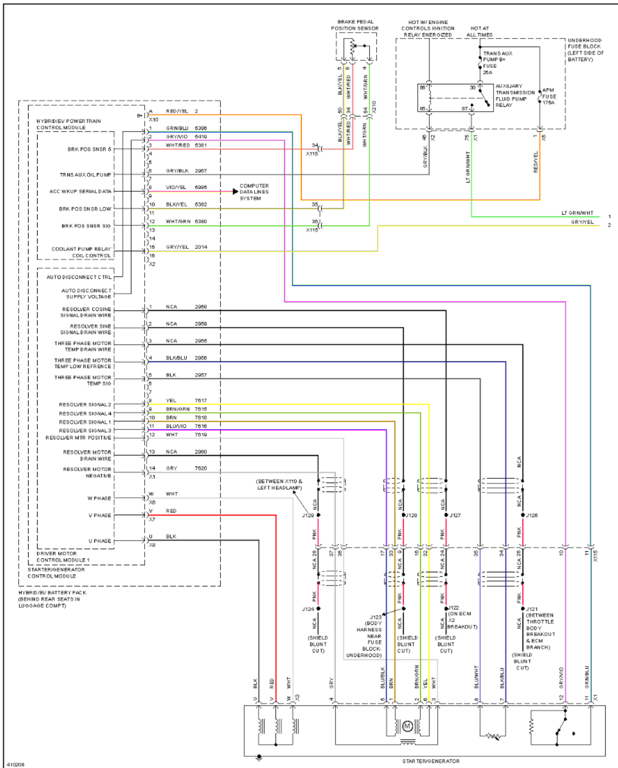
Fig. 41: 2.4L VIN R, Hybrid System Circuit (1 of 4)
