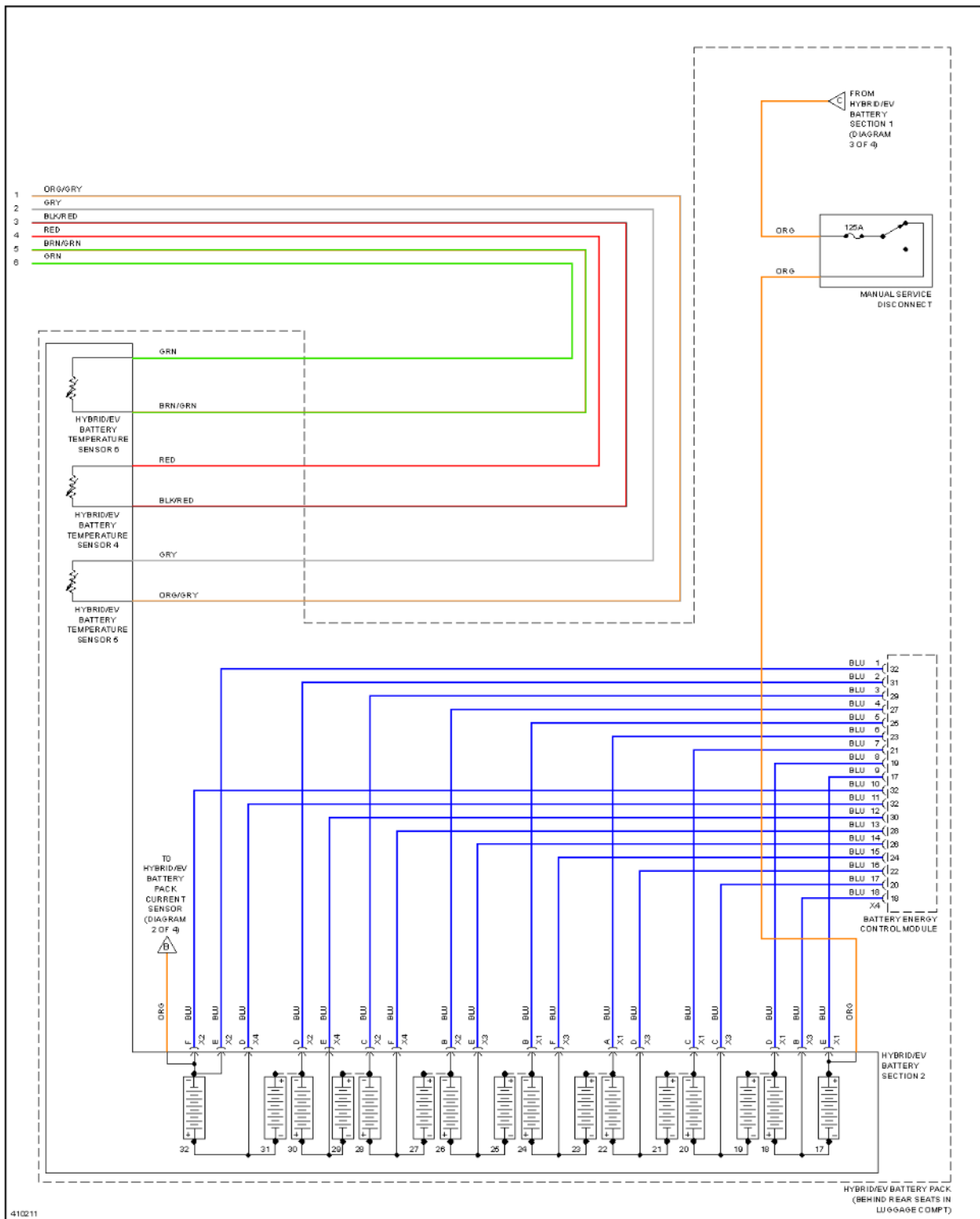
Fig. 44: 2.4L VIN R, Hybrid System Circuit (4 of 4)
