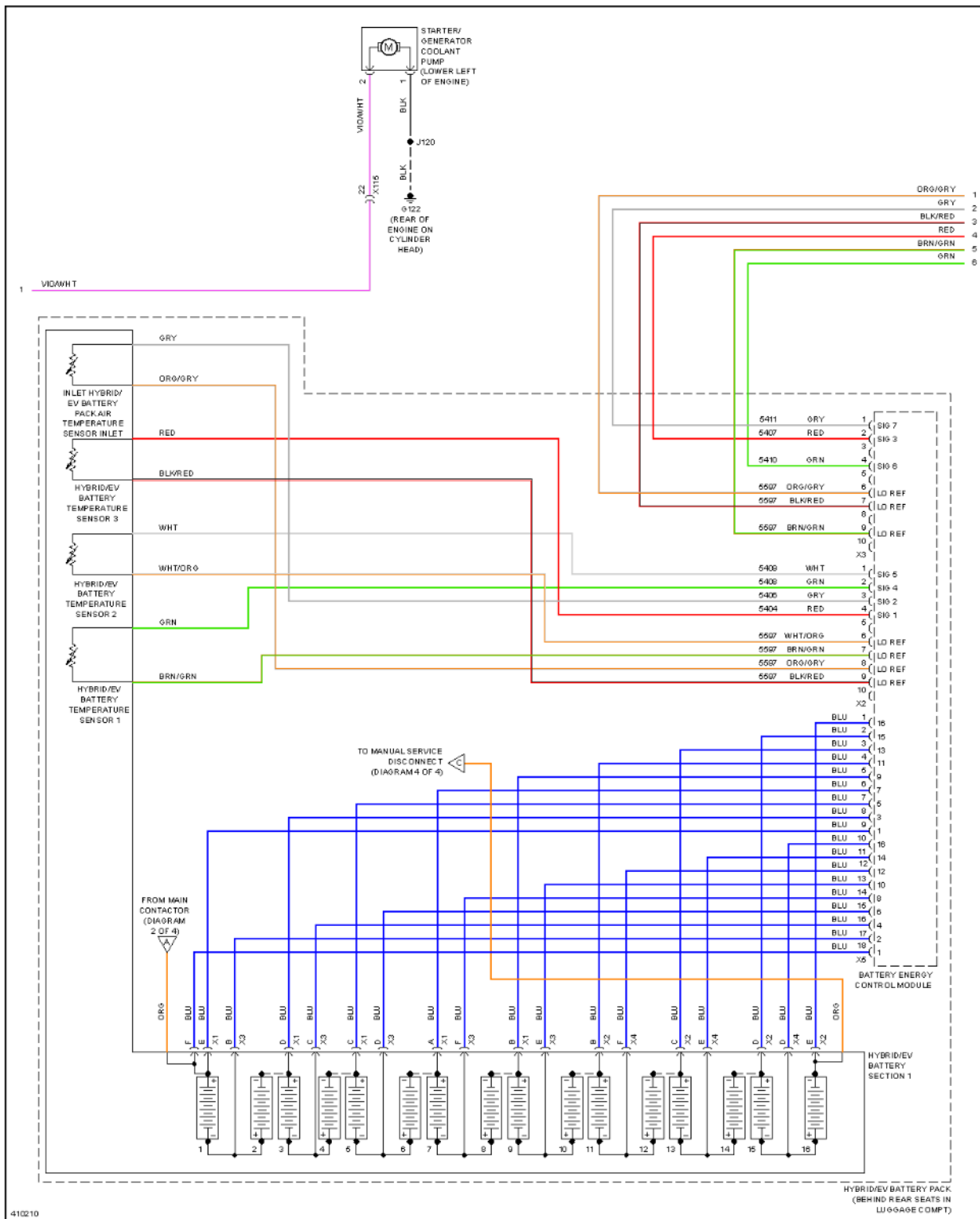
Fig. 43: 2.4L VIN R, Hybrid System Circuit (3 of 4)
