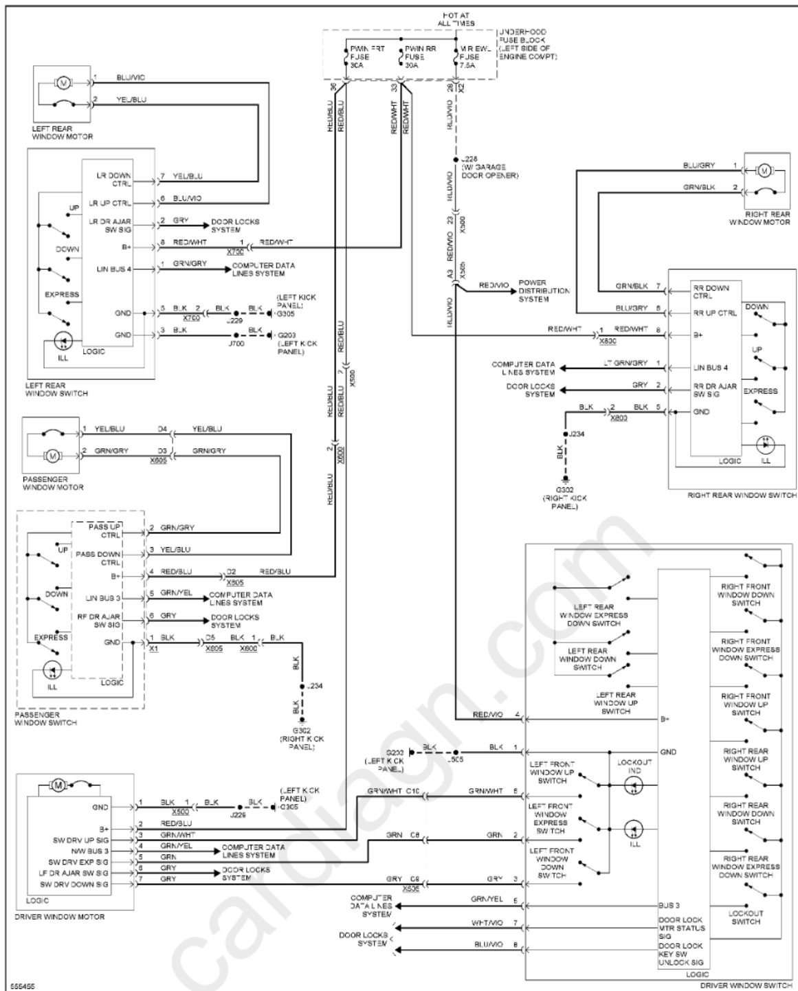
Fig. 109: Power Windows Circuit
