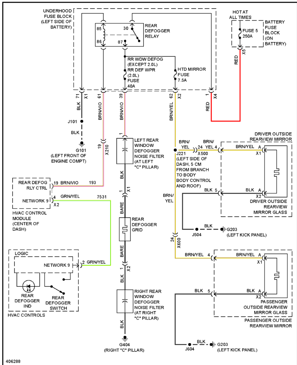
Fig. 27: Defoggers Circuit
