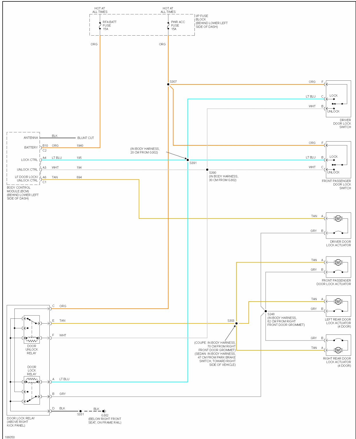
Fig. 24: Power Door Locks Circuit, W/ Keyless Entry
