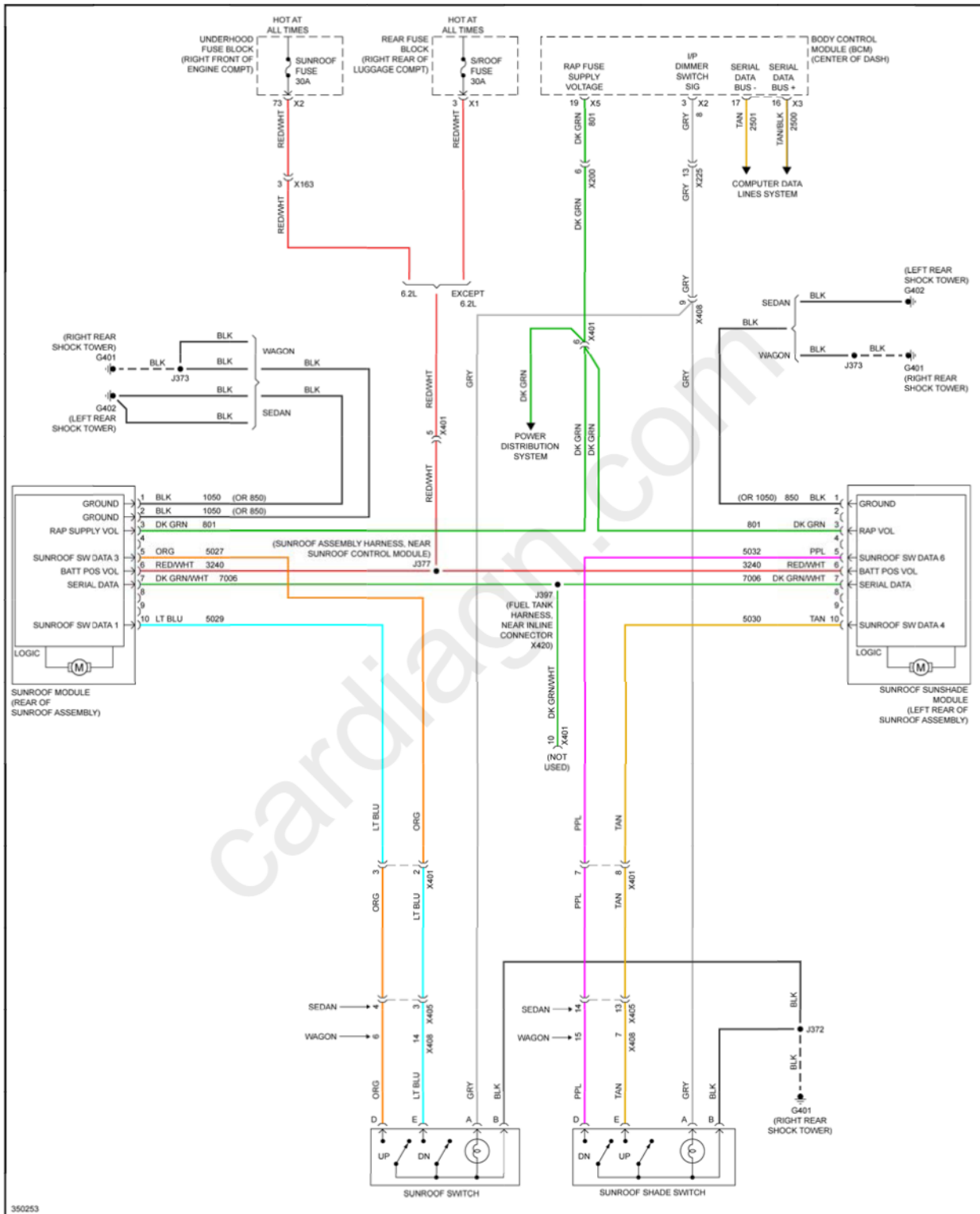
Fig. 97: Power Top/Sunroof Circuit, Sedan & Wagon
